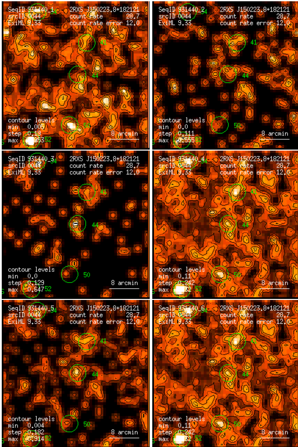
Figure 44: RASS 931440: detection 0044: band rate images, Gaussian filter: (1) PSPC channels 11 – 41, (2) 52 – 90, (3) 91 – 201, (4) 11 – 235, (5) 52 – 201, (6) 11 – 201. Broad band rates in counts/ks. Band rate contour levels in counts/ks/arcmin 2 .
