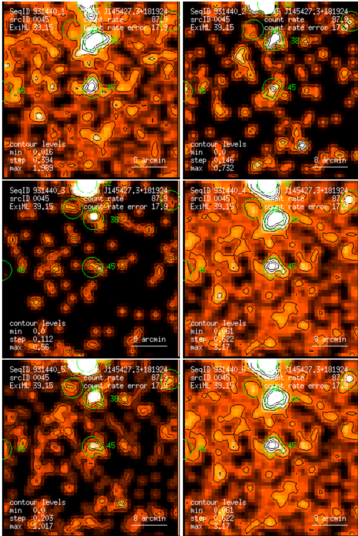
Figure 45: RASS 931440: detection 0045: band rate images, Gaussian filter: (1) PSPC channels 11 – 41, (2) 52 – 90, (3) 91 – 201, (4) 11 – 235, (5) 52 – 201, (6) 11 – 201. Broad band rates in counts/ks. Band rate contour levels in counts/ks/arcmin 2 .
