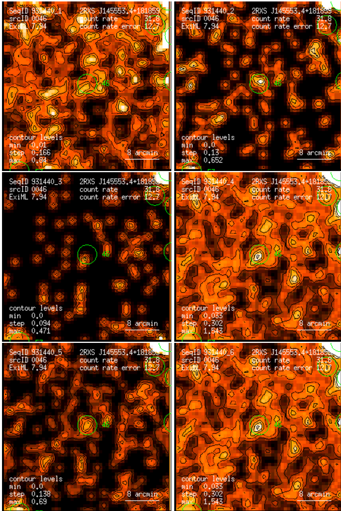
Figure 46: RASS 931440: detection 0046: band rate images, Gaussian filter: (1) PSPC channels 11 – 41, (2) 52 – 90, (3) 91 – 201, (4) 11 – 235, (5) 52 – 201, (6) 11 – 201. Broad band rates in counts/ks. Band rate contour levels in counts/ks/arcmin 2 .
