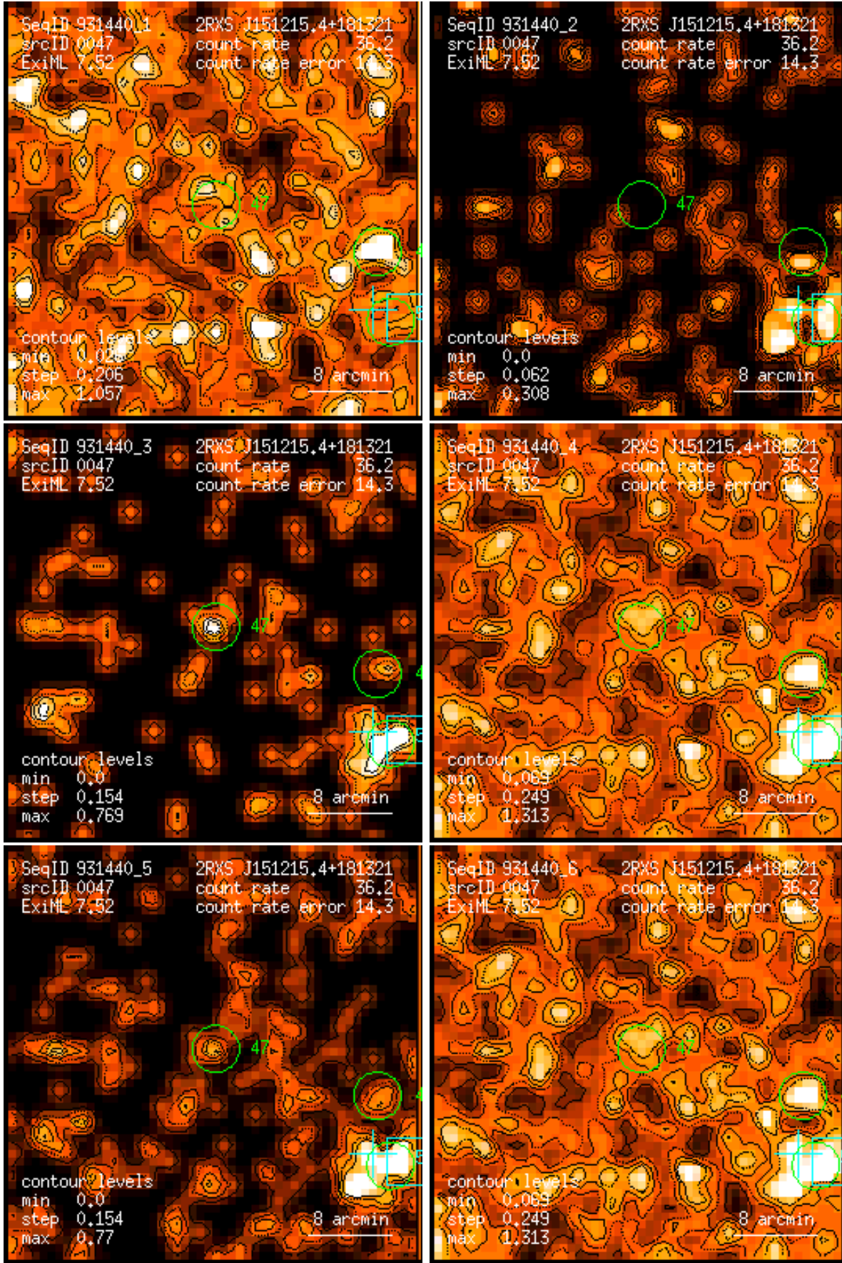
Figure 47: RASS 931440: detection 0047: band rate images, Gaussian filter: (1) PSPC channels 11 – 41, (2) 52 – 90, (3) 91 – 201, (4) 11 – 235, (5) 52 – 201, (6) 11 – 201. Broad band rates in counts/ks. Band rate contour levels in counts/ks/arcmin 2 .
