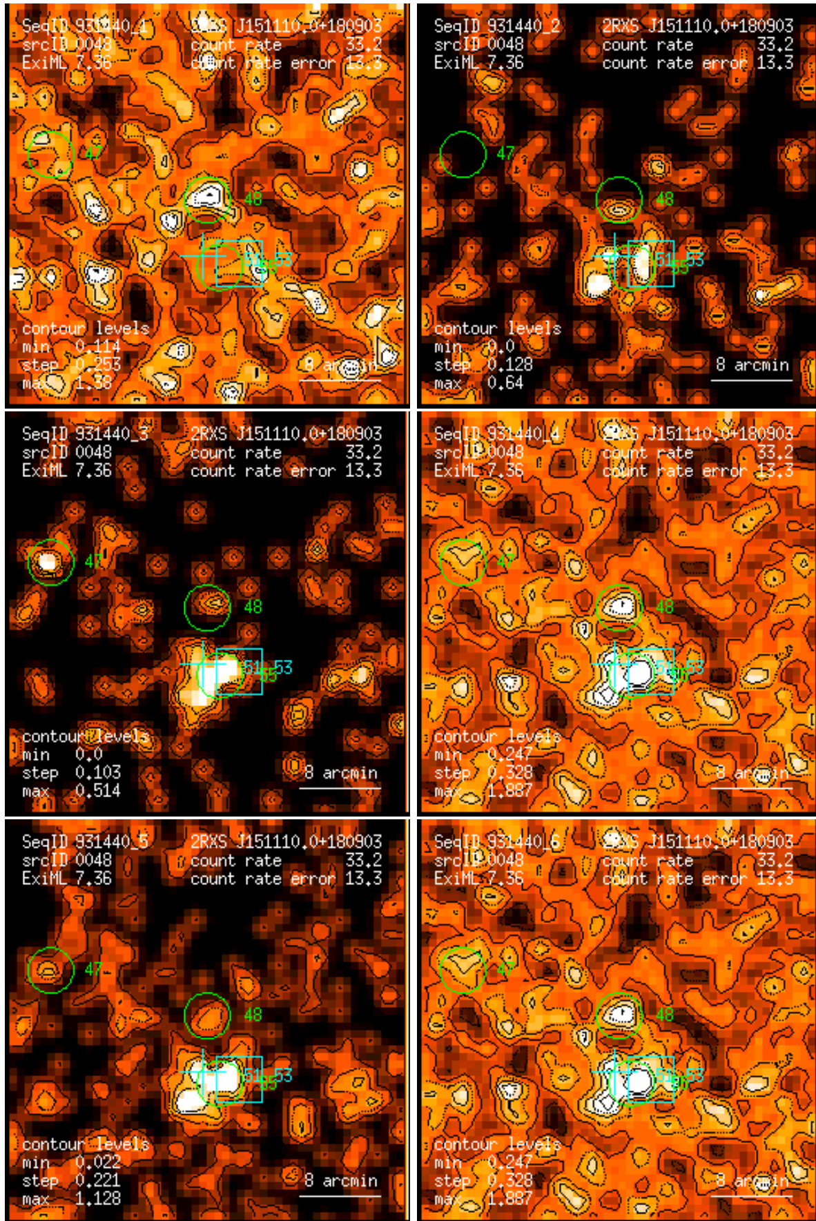
Figure 48: RASS 931440: detection 0048: band rate images, Gaussian filter: (1) PSPC channels 11 – 41, (2) 52 – 90, (3) 91 – 201, (4) 11 – 235, (5) 52 – 201, (6) 11 – 201. Broad band rates in counts/ks. Band rate contour levels in counts/ks/arcmin 2 .
