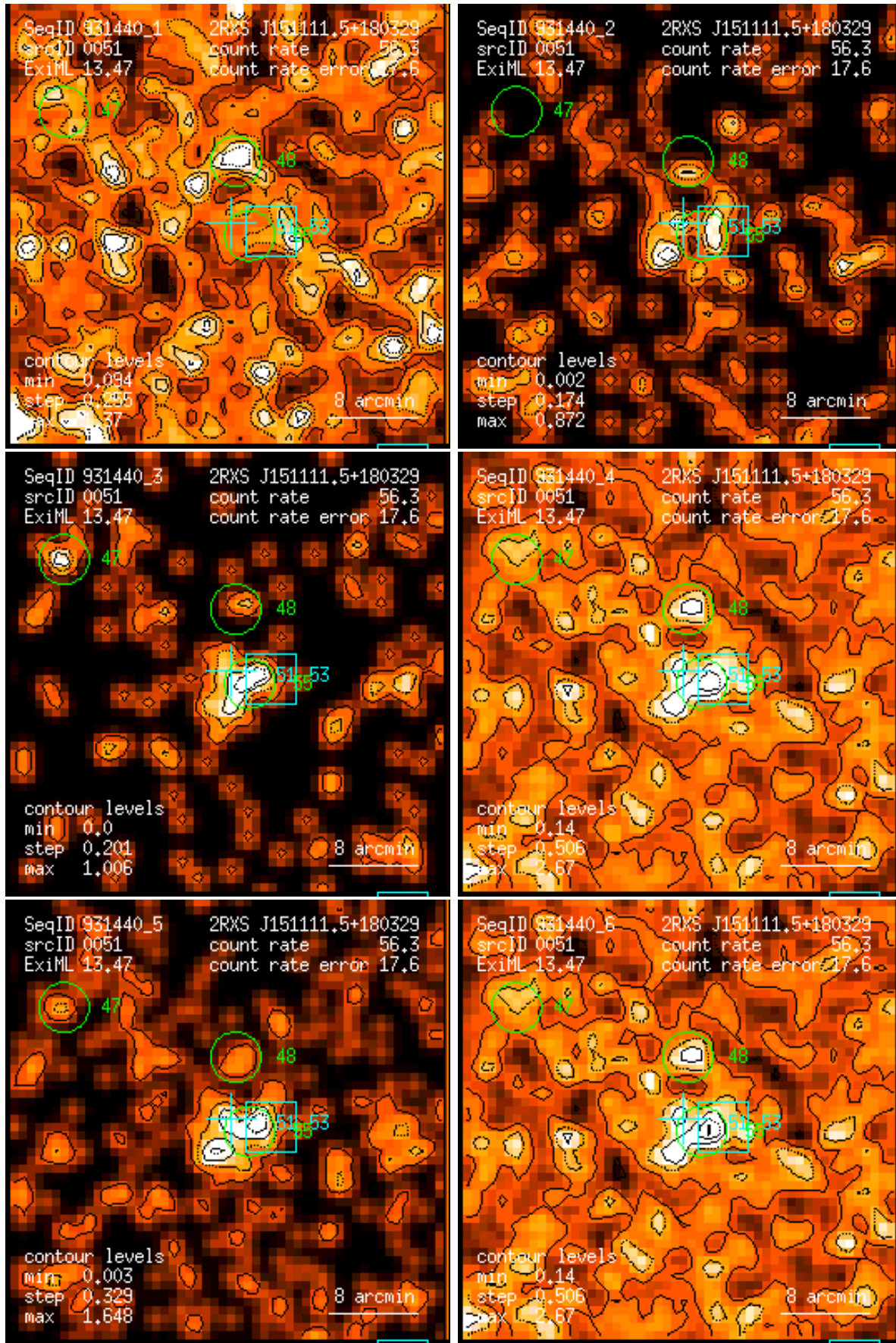
Figure 51: RASS 931440: detection 0051: band rate images, Gaussian filter: (1) PSPC channels 11 – 41, (2) 52 – 90, (3) 91 – 201, (4) 11 – 235, (5) 52 – 201, (6) 11 – 201. Broad band rates in counts/ks. Band rate contour levels in counts/ks/arcmin 2 .
