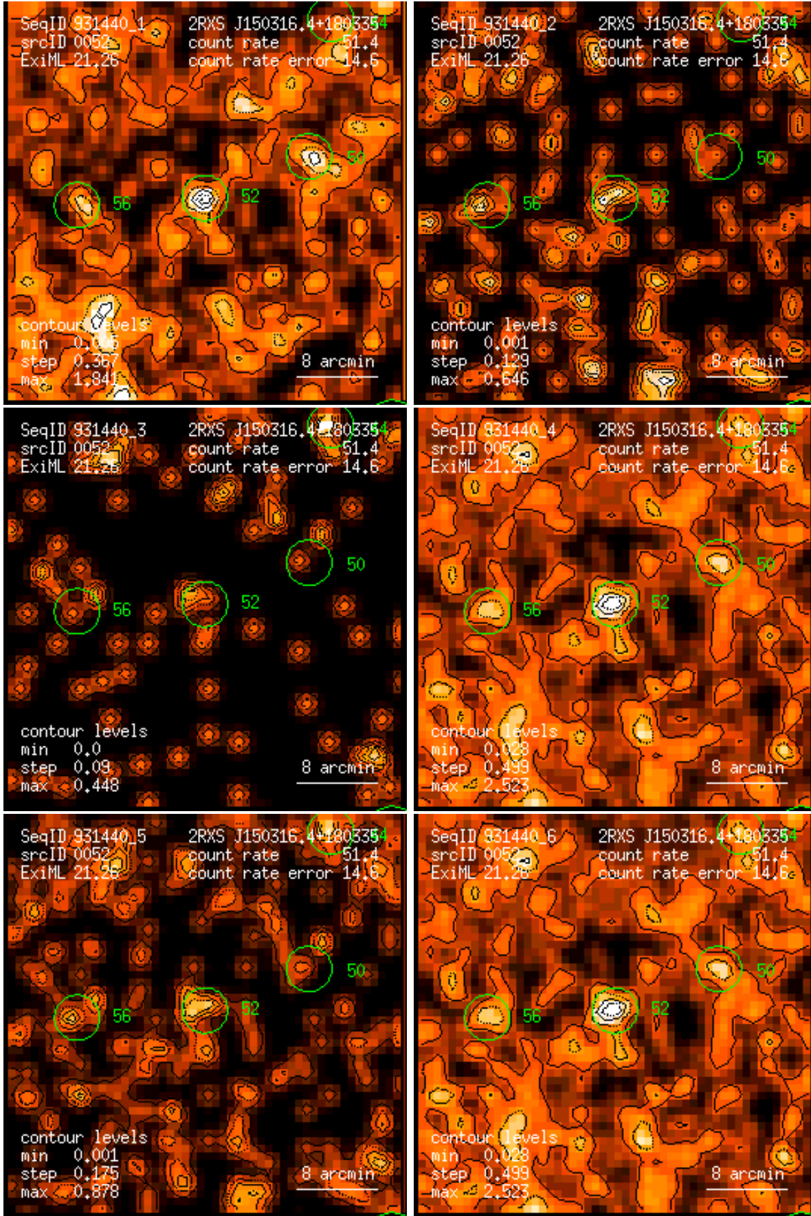
Figure 52: RASS 931440: detection 0052: band rate images, Gaussian filter: (1) PSPC channels 11 – 41, (2) 52 – 90, (3) 91 – 201, (4) 11 – 235, (5) 52 – 201, (6) 11 – 201. Broad band rates in counts/ks. Band rate contour levels in counts/ks/arcmin 2 .
