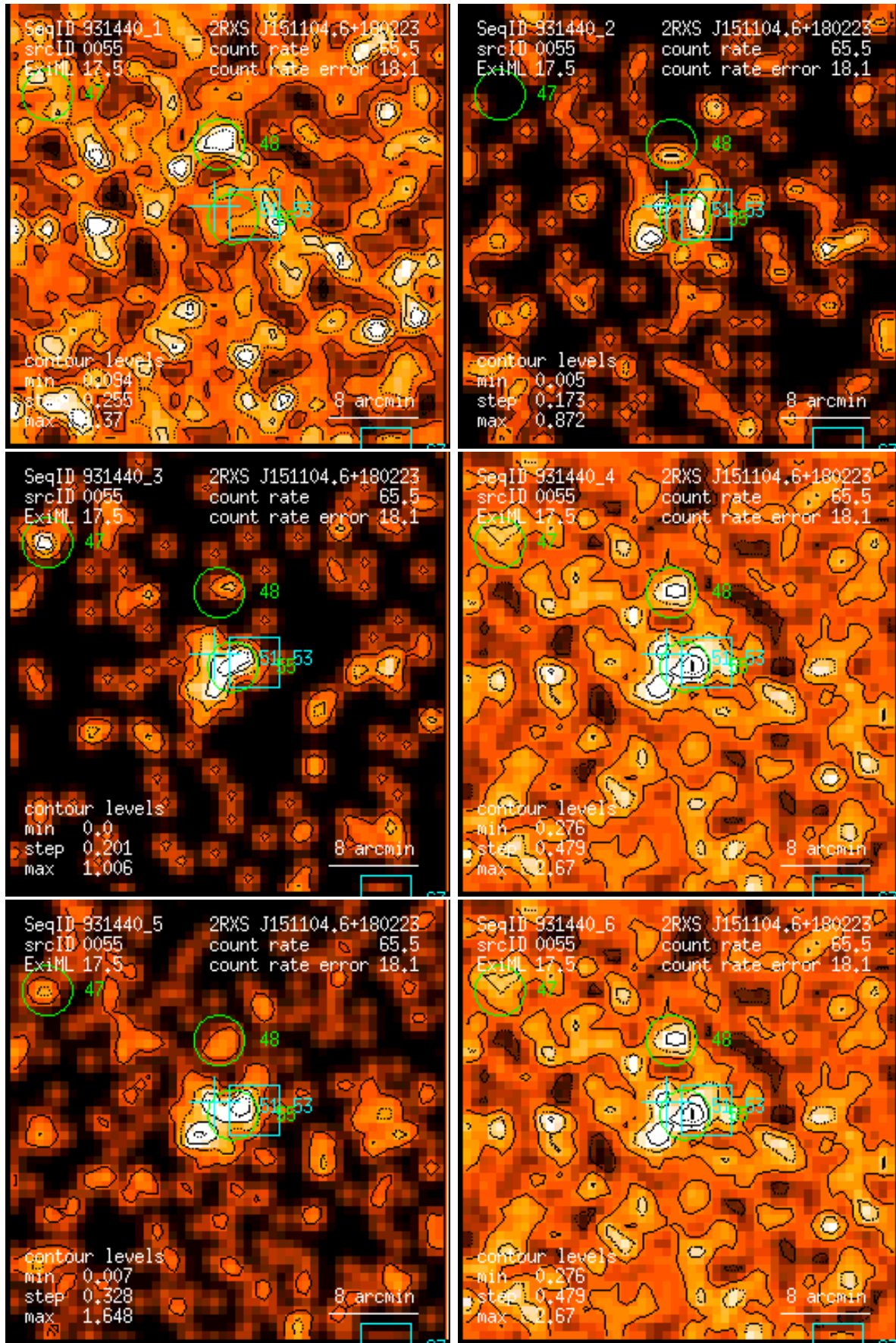
Figure 55: RASS 931440: detection 0055: band rate images, Gaussian filter: (1) PSPC channels 11 – 41, (2) 52 – 90, (3) 91 – 201, (4) 11 – 235, (5) 52 – 201, (6) 11 – 201. Broad band rates in counts/ks. Band rate contour levels in counts/ks/arcmin 2 .
