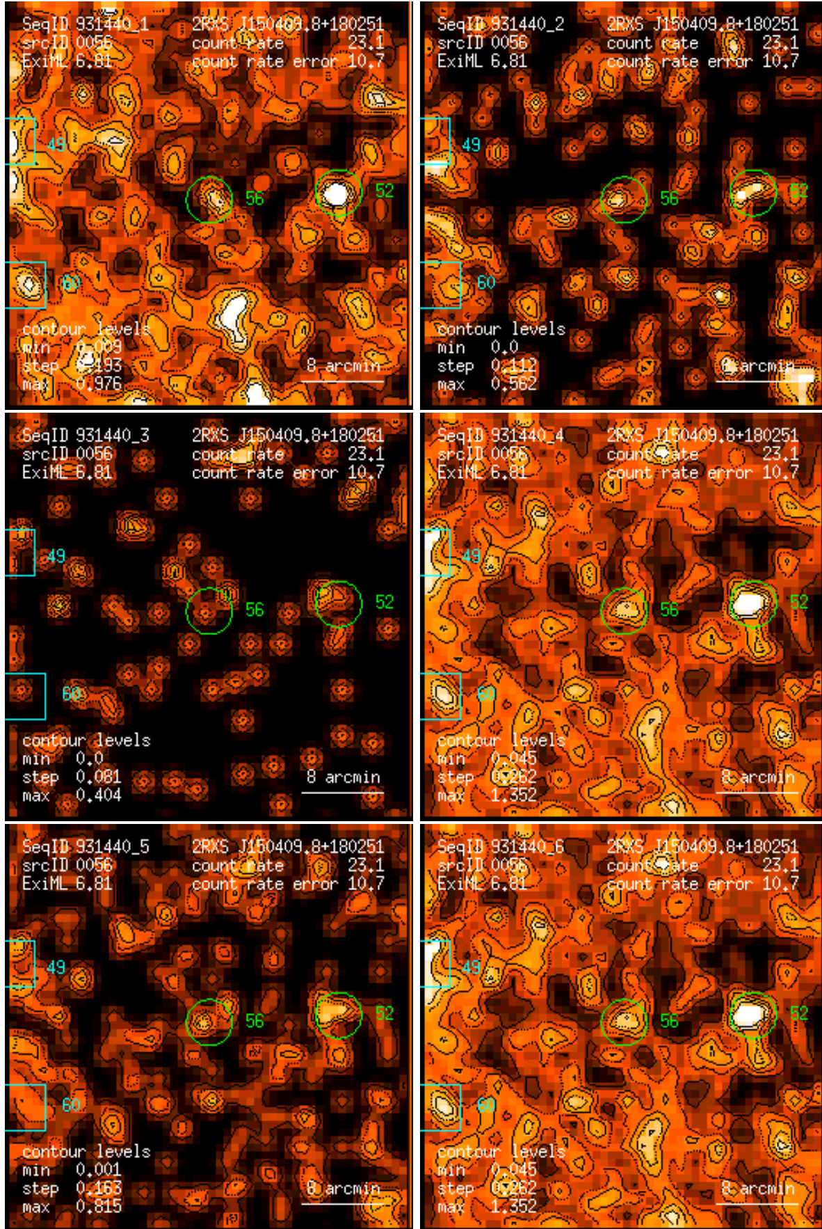
Figure 56: RASS 931440: detection 0056: band rate images, Gaussian filter: (1) PSPC channels 11 – 41, (2) 52 – 90, (3) 91 – 201, (4) 11 – 235, (5) 52 – 201, (6) 11 – 201. Broad band rates in counts/ks. Band rate contour levels in counts/ks/arcmin 2 .
