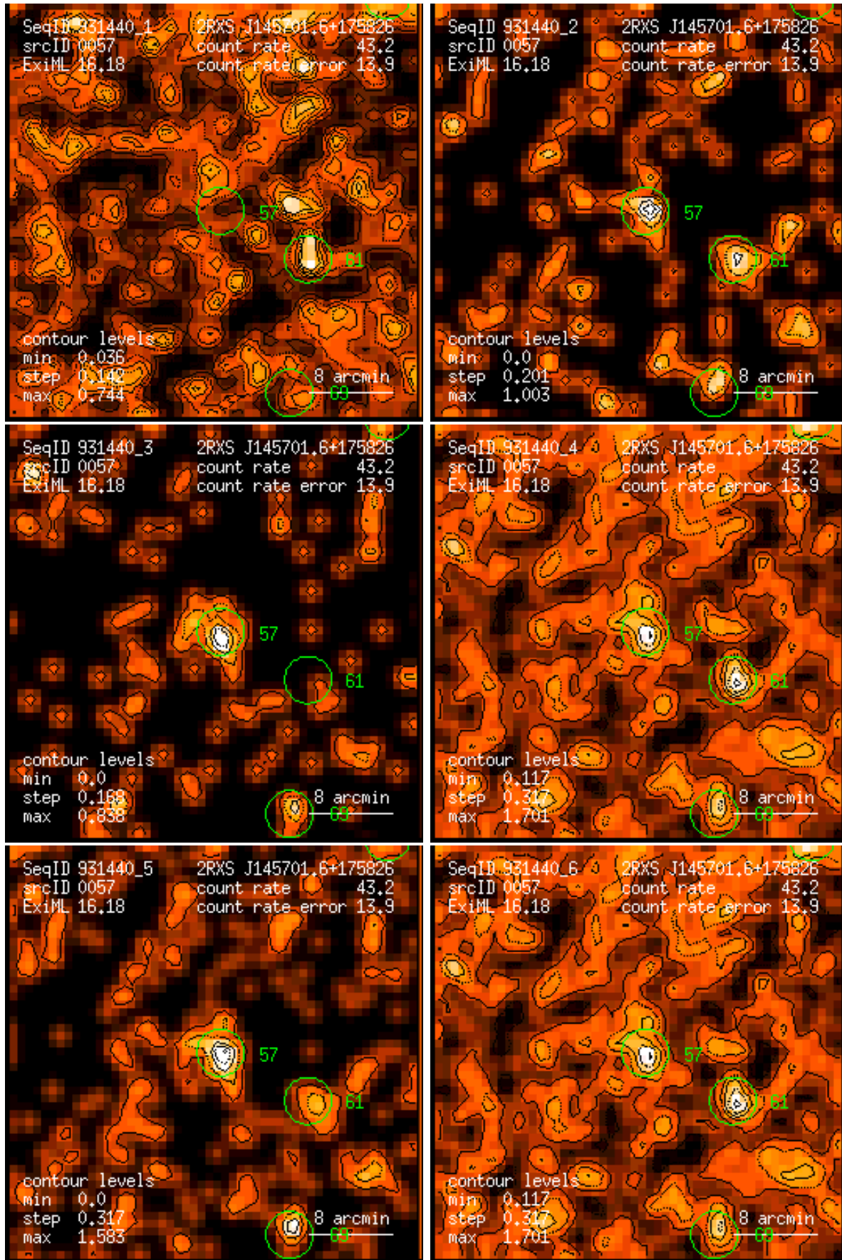
Figure 57: RASS 931440: detection 0057: band rate images, Gaussian filter: (1) PSPC channels 11 – 41, (2) 52 – 90, (3) 91 – 201, (4) 11 – 235, (5) 52 – 201, (6) 11 – 201. Broad band rates in counts/ks. Band rate contour levels in counts/ks/arcmin 2 .
