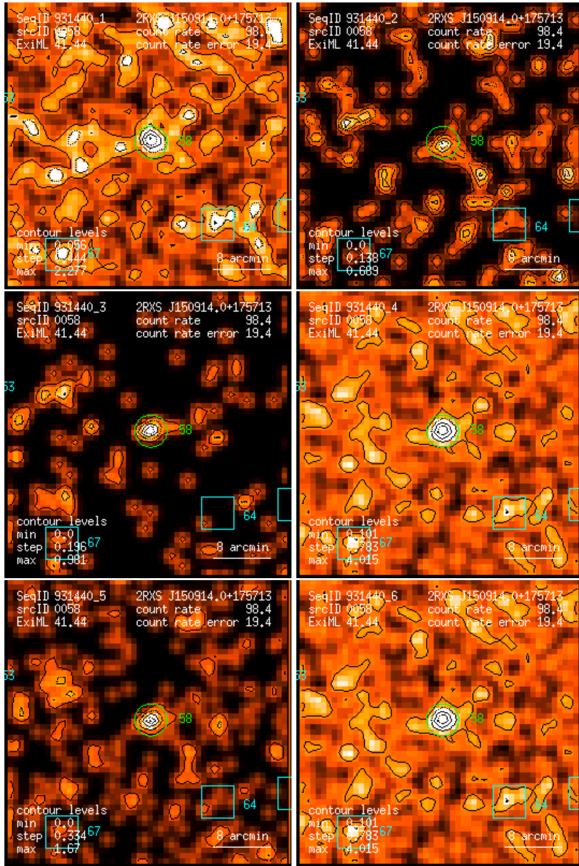
Figure 58: RASS 931440: detection 0058: band rate images, Gaussian filter: (1) PSPC channels 11 – 41, (2) 52 – 90, (3) 91 – 201, (4) 11 – 235, (5) 52 – 201, (6) 11 – 201. Broad band rates in counts/ks. Band rate contour levels in counts/ks/arcmin 2 .
