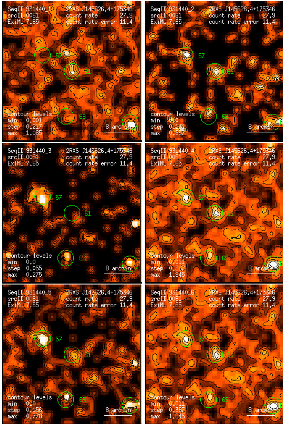
Figure 61: RASS 931440: detection 0061: band rate images, Gaussian filter: (1) PSPC channels 11 – 41, (2) 52 – 90, (3) 91 – 201, (4) 11 – 235, (5) 52 – 201, (6) 11 – 201. Broad band rates in counts/ks. Band rate contour levels in counts/ks/arcmin 2 .
