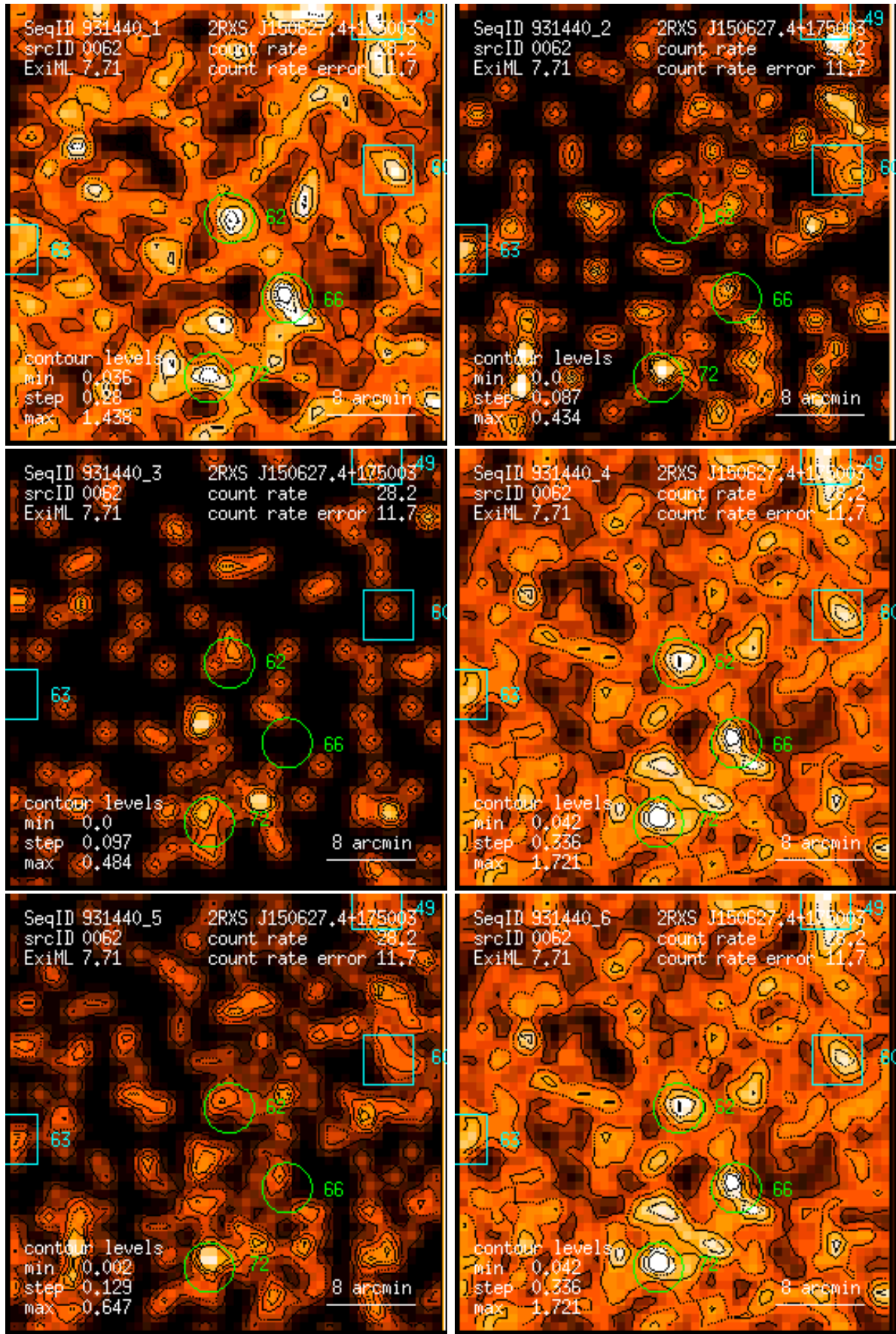
Figure 62: RASS 931440: detection 0062: band rate images, Gaussian filter: (1) PSPC channels 11 – 41, (2) 52 – 90, (3) 91 – 201, (4) 11 – 235, (5) 52 – 201, (6) 11 – 201. Broad band rates in counts/ks. Band rate contour levels in counts/ks/arcmin 2 .
