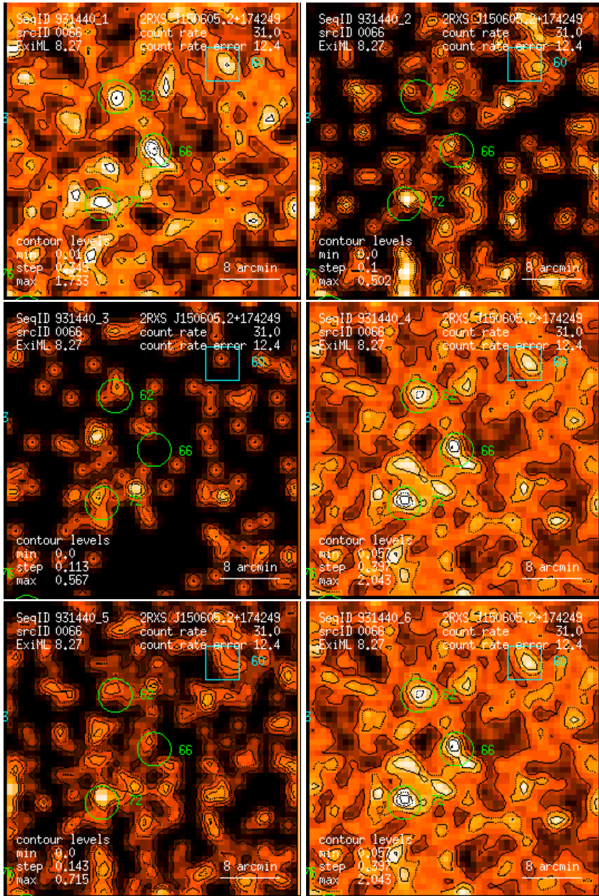
Figure 66: RASS 931440: detection 0066: band rate images, Gaussian filter: (1) PSPC channels 11 – 41, (2) 52 – 90, (3) 91 – 201, (4) 11 – 235, (5) 52 – 201, (6) 11 – 201. Broad band rates in counts/ks. Band rate contour levels in counts/ks/arcmin 2 .
