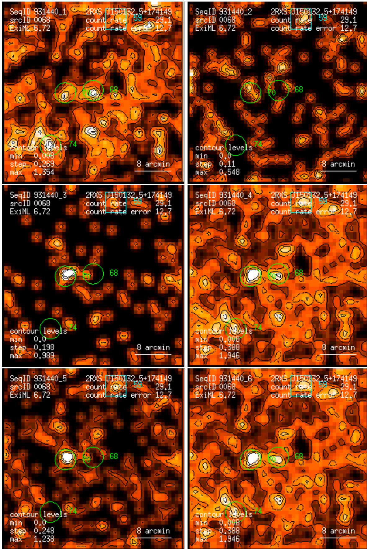
Figure 68: RASS 931440: detection 0068: band rate images, Gaussian filter: (1) PSPC channels 11 – 41, (2) 52 – 90, (3) 91 – 201, (4) 11 – 235, (5) 52 – 201, (6) 11 – 201. Broad band rates in counts/ks. Band rate contour levels in counts/ks/arcmin 2 .
