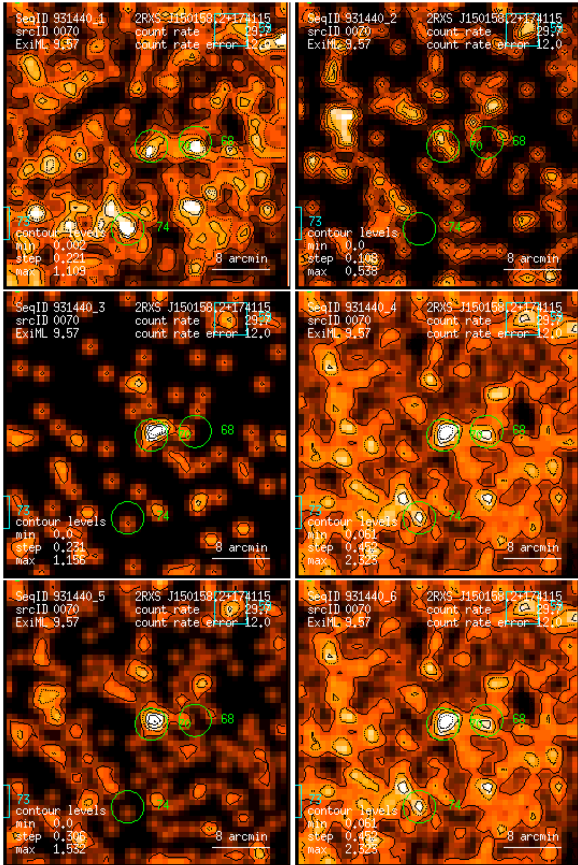
Figure 70: RASS 931440: detection 0070: band rate images, Gaussian filter: (1) PSPC channels 11 – 41, (2) 52 – 90, (3) 91 – 201, (4) 11 – 235, (5) 52 – 201, (6) 11 – 201. Broad band rates in counts/ks. Band rate contour levels in counts/ks/arcmin 2 .
