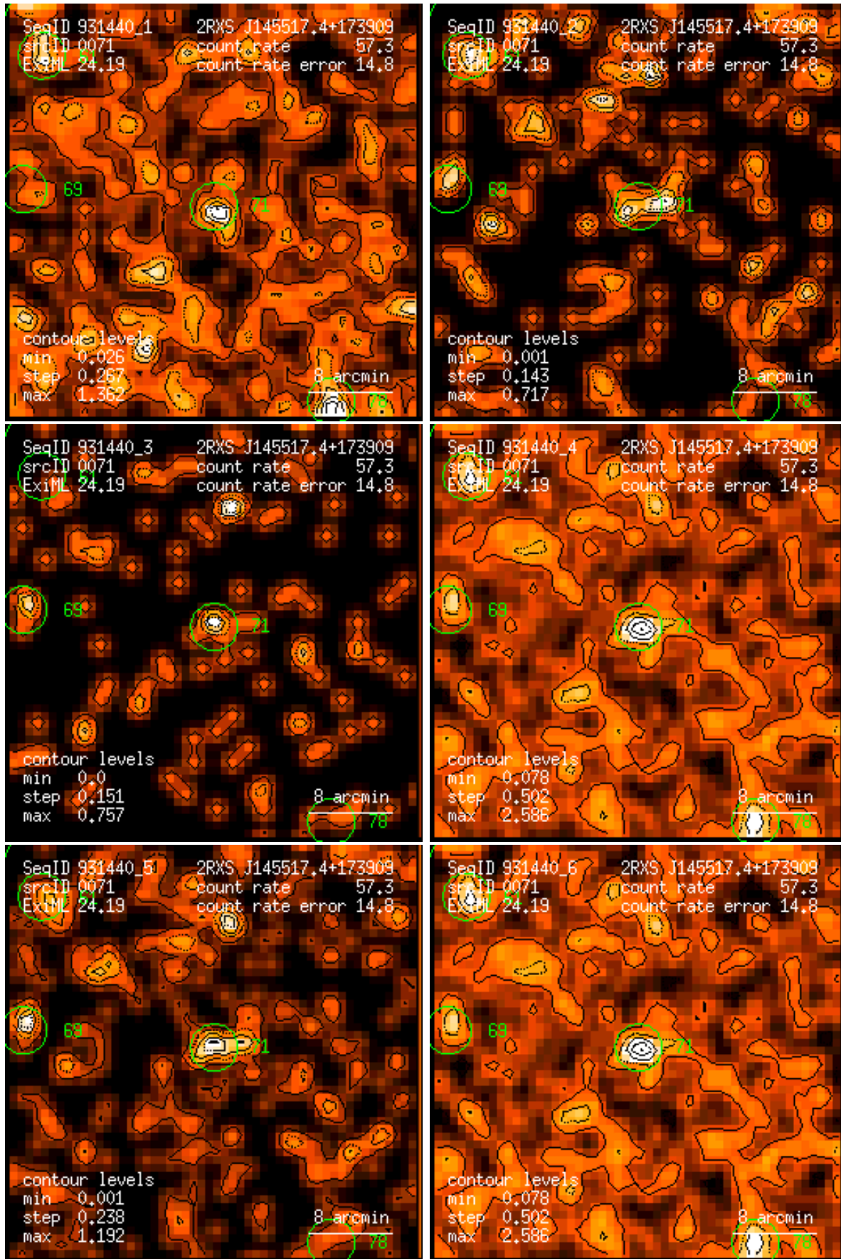
Figure 71: RASS 931440: detection 0071: band rate images, Gaussian filter: (1) PSPC channels 11 – 41, (2) 52 – 90, (3) 91 – 201, (4) 11 – 235, (5) 52 – 201, (6) 11 – 201. Broad band rates in counts/ks. Band rate contour levels in counts/ks/arcmin 2 .
