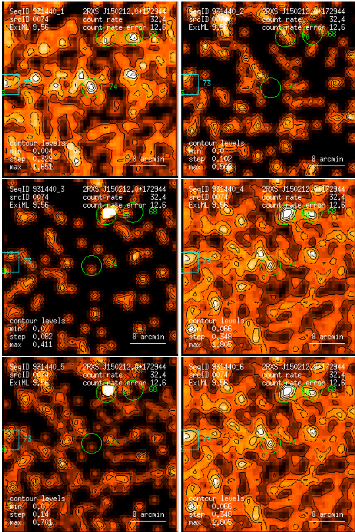
Figure 74: RASS 931440: detection 0074: band rate images, Gaussian filter: (1) PSPC channels 11 – 41, (2) 52 – 90, (3) 91 – 201, (4) 11 – 235, (5) 52 – 201, (6) 11 – 201. Broad band rates in counts/ks. Band rate contour levels in counts/ks/arcmin 2 .
