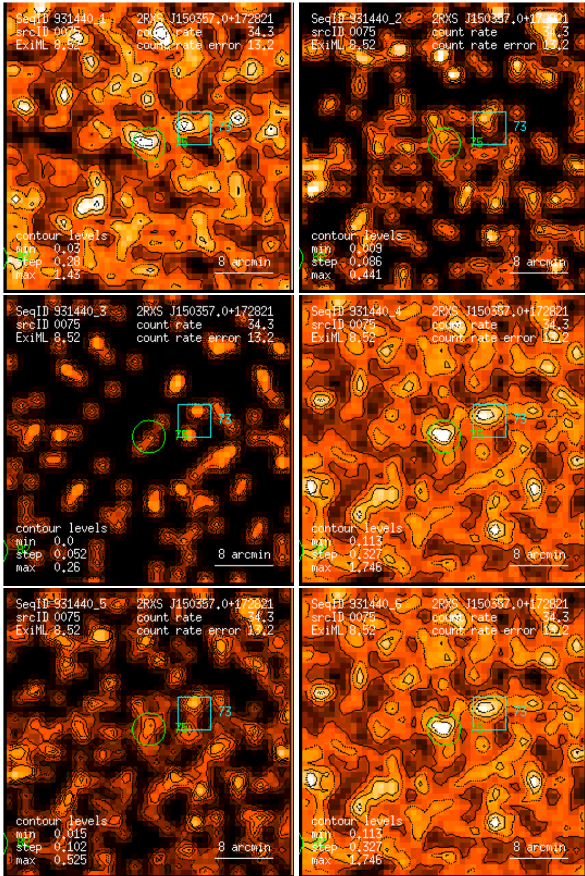
Figure 75: RASS 931440: detection 0075: band rate images, Gaussian filter: (1) PSPC channels 11 – 41, (2) 52 – 90, (3) 91 – 201, (4) 11 – 235, (5) 52 – 201, (6) 11 – 201. Broad band rates in counts/ks. Band rate contour levels in counts/ks/arcmin 2 .
