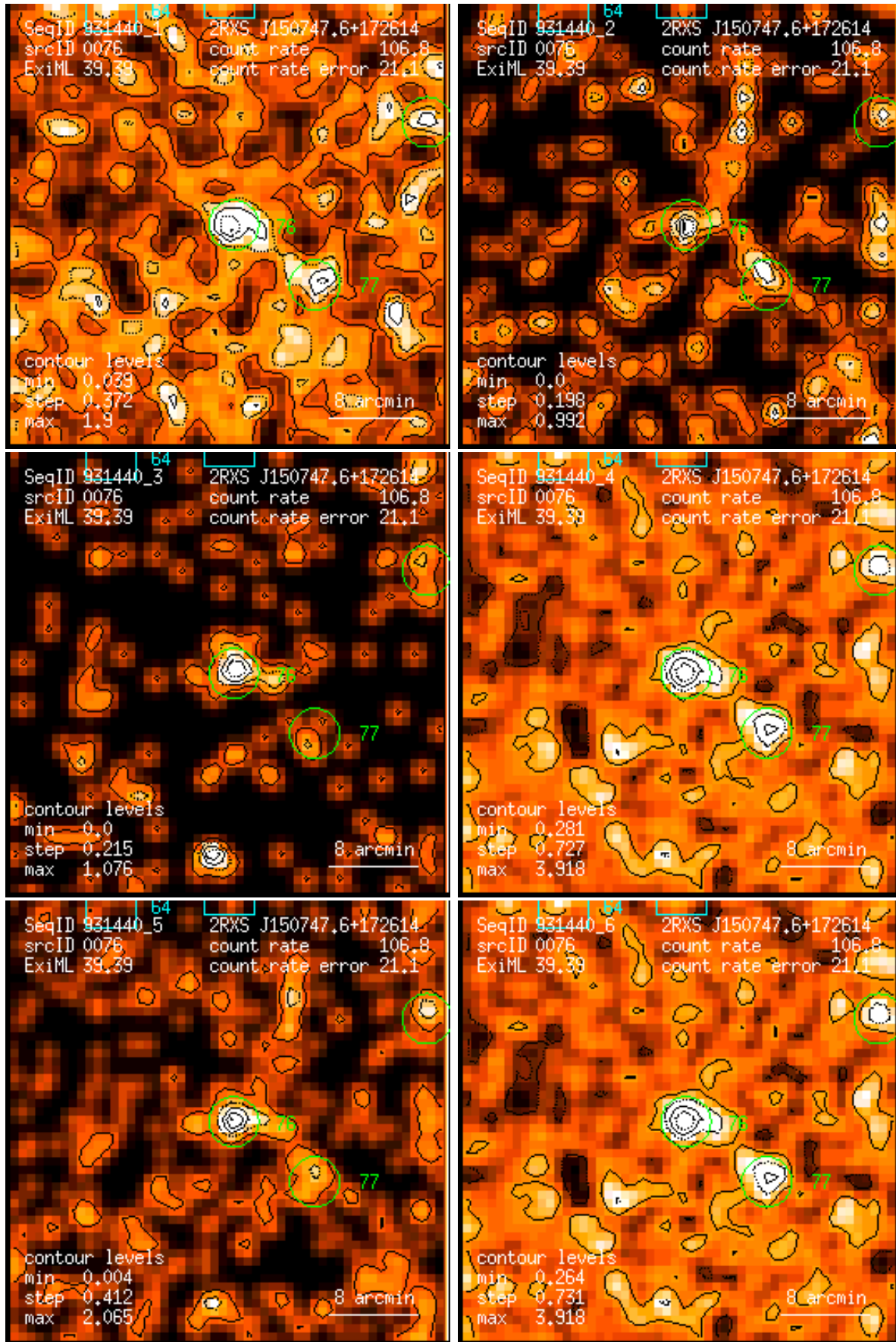
Figure 76: RASS 931440: detection 0076: band rate images, Gaussian filter: (1) PSPC channels 11 – 41, (2) 52 – 90, (3) 91 – 201, (4) 11 – 235, (5) 52 – 201, (6) 11 – 201. Broad band rates in counts/ks. Band rate contour levels in counts/ks/arcmin 2 .
