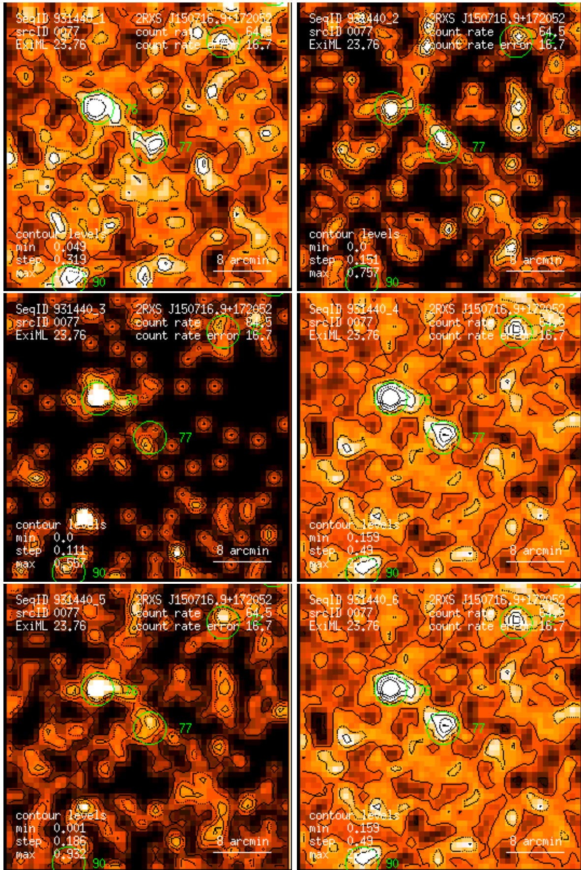
Figure 77: RASS 931440: detection 0077: band rate images, Gaussian filter: (1) PSPC channels 11 – 41, (2) 52 – 90, (3) 91 – 201, (4) 11 – 235, (5) 52 – 201, (6) 11 – 201. Broad band rates in counts/ks. Band rate contour levels in counts/ks/arcmin 2 .
