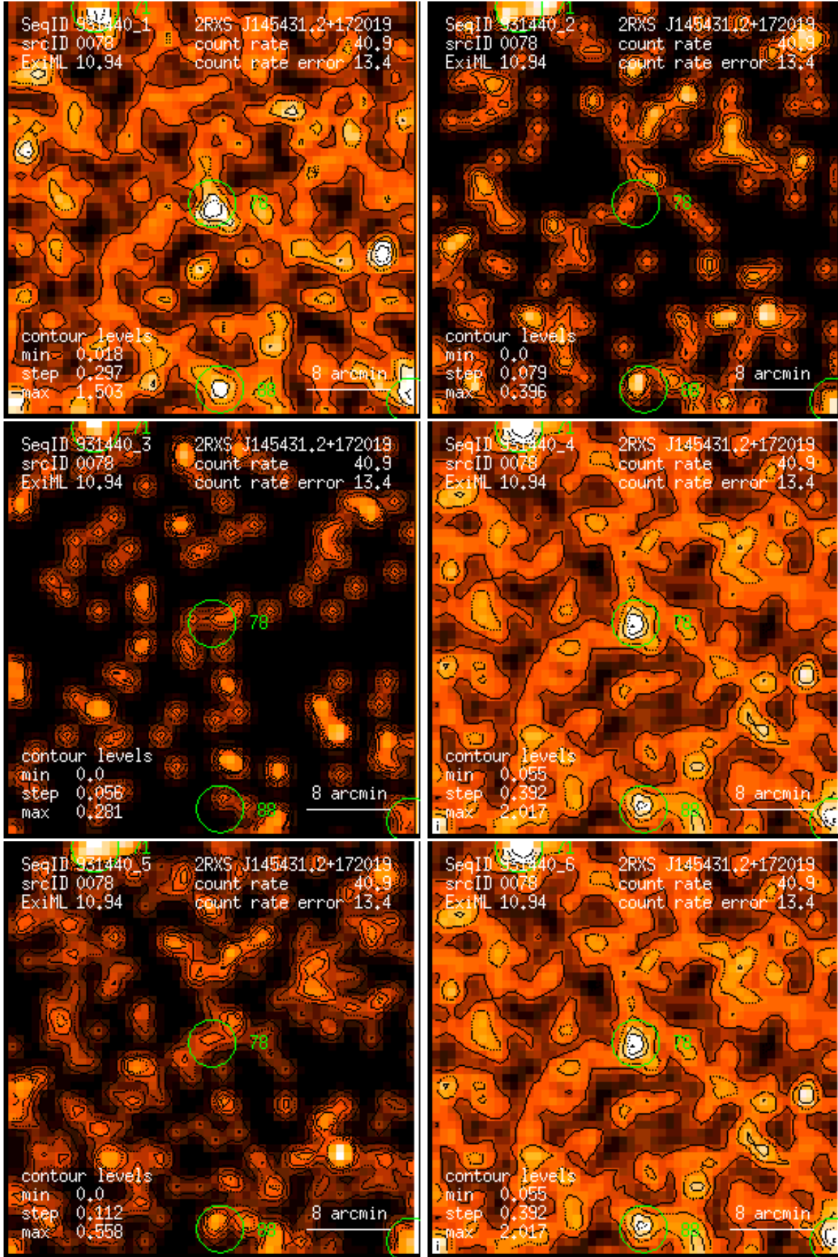
Figure 78: RASS 931440: detection 0078: band rate images, Gaussian filter: (1) PSPC channels 11 – 41, (2) 52 – 90, (3) 91 – 201, (4) 11 – 235, (5) 52 – 201, (6) 11 – 201. Broad band rates in counts/ks. Band rate contour levels in counts/ks/arcmin 2 .
