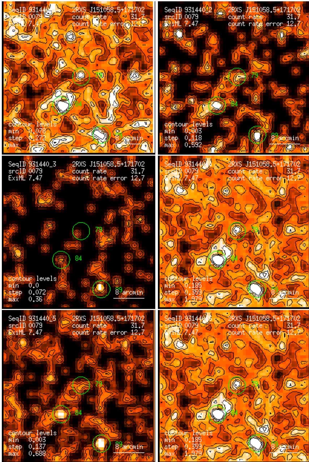
Figure 79: RASS 931440: detection 0079: band rate images, Gaussian filter: (1) PSPC channels 11 – 41, (2) 52 – 90, (3) 91 – 201, (4) 11 – 235, (5) 52 – 201, (6) 11 – 201. Broad band rates in counts/ks. Band rate contour levels in counts/ks/arcmin 2 .
