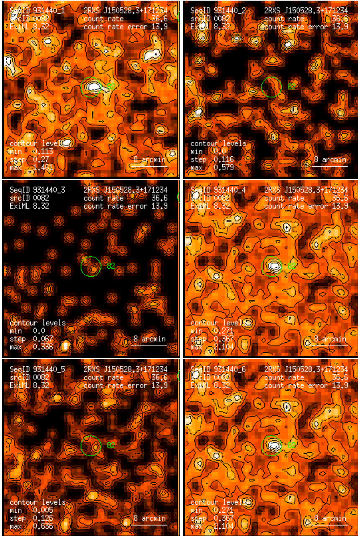
Figure 82: RASS 931440: detection 0082: band rate images, Gaussian filter: (1) PSPC channels 11 – 41, (2) 52 – 90, (3) 91 – 201, (4) 11 – 235, (5) 52 – 201, (6) 11 – 201. Broad band rates in counts/ks. Band rate contour levels in counts/ks/arcmin 2 .
