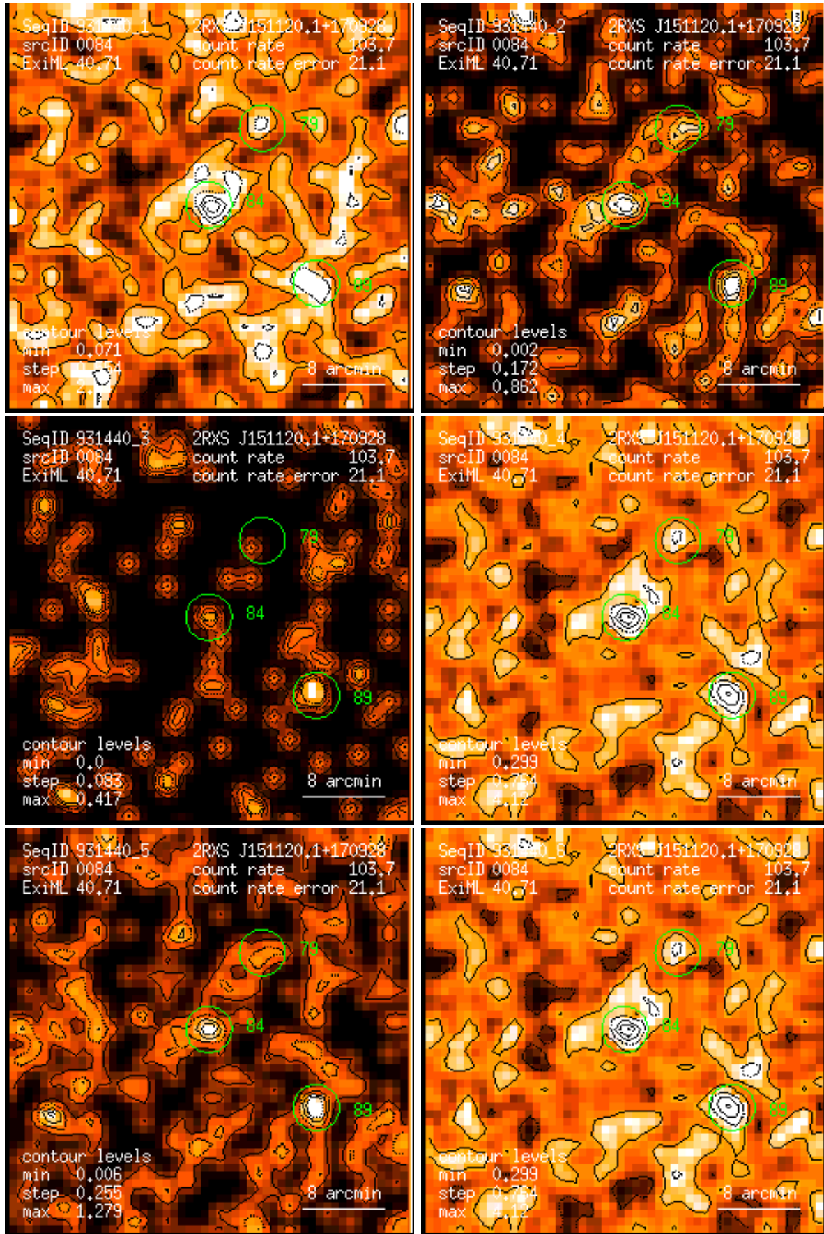
Figure 84: RASS 931440: detection 0084: band rate images, Gaussian filter: (1) PSPC channels 11 – 41, (2) 52 – 90, (3) 91 – 201, (4) 11 – 235, (5) 52 – 201, (6) 11 – 201. Broad band rates in counts/ks. Band rate contour levels in counts/ks/arcmin 2 .
