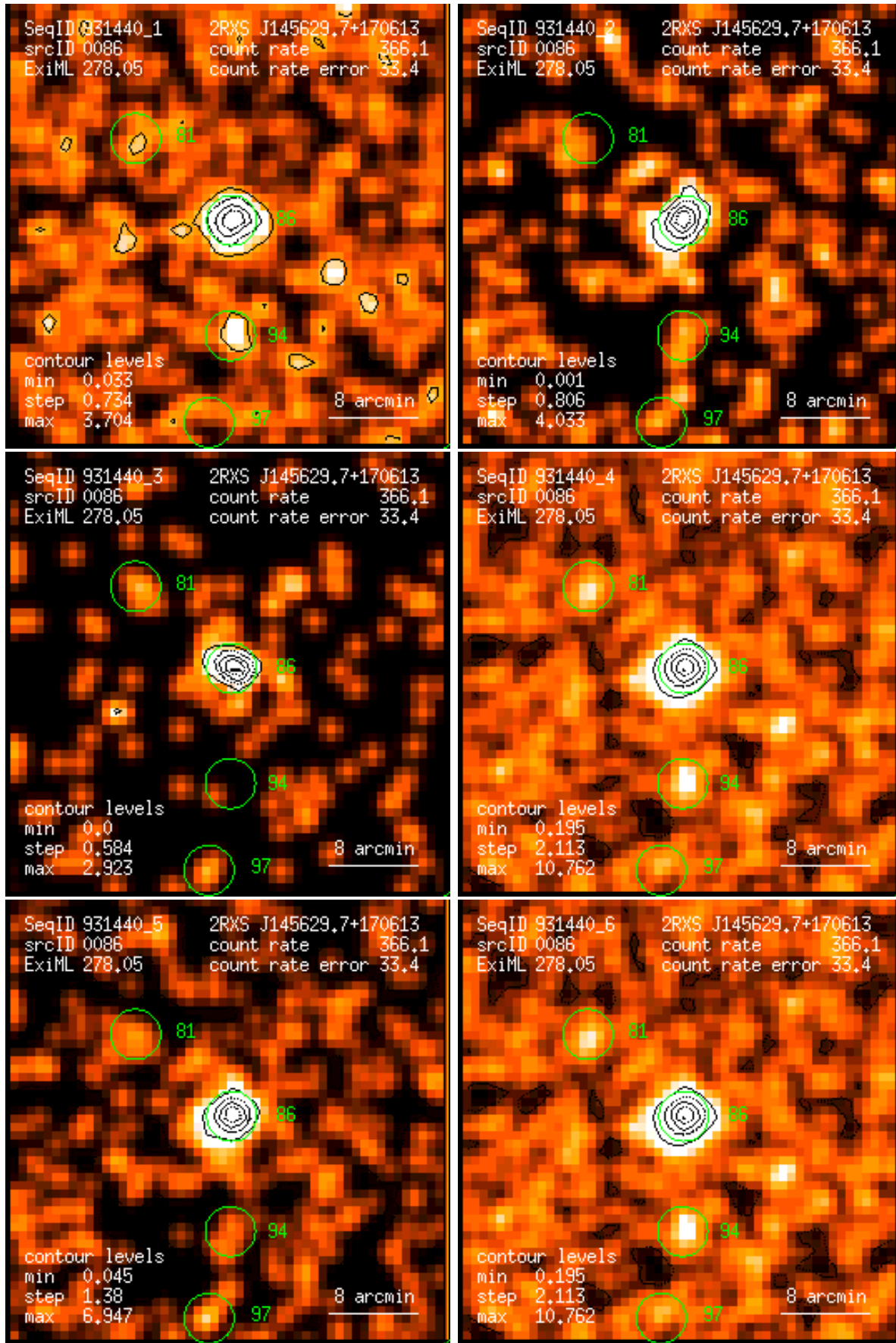
Figure 86: RASS 931440: detection 0086: band rate images, Gaussian filter: (1) PSPC channels 11 – 41, (2) 52 – 90, (3) 91 – 201, (4) 11 – 235, (5) 52 – 201, (6) 11 – 201. Broad band rates in counts/ks. Band rate contour levels in counts/ks/arcmin 2 .
