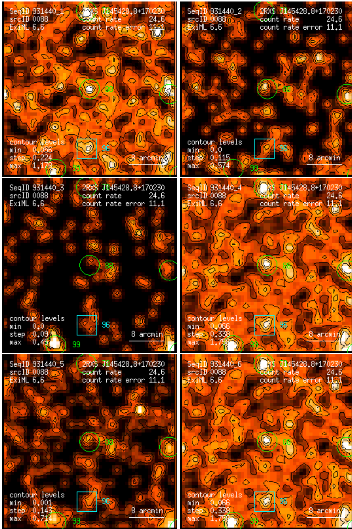
Figure 88: RASS 931440: detection 0088: band rate images, Gaussian filter: (1) PSPC channels 11 – 41, (2) 52 – 90, (3) 91 – 201, (4) 11 – 235, (5) 52 – 201, (6) 11 – 201. Broad band rates in counts/ks. Band rate contour levels in counts/ks/arcmin 2 .
