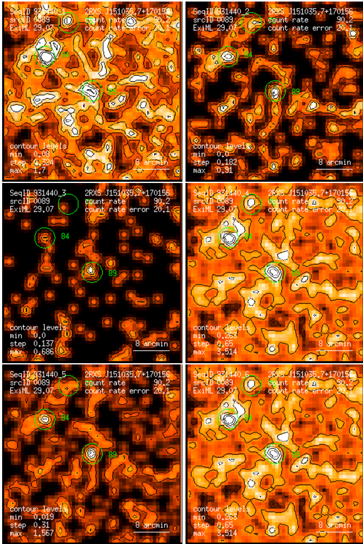
Figure 89: RASS 931440: detection 0089: band rate images, Gaussian filter: (1) PSPC channels 11 – 41, (2) 52 – 90, (3) 91 – 201, (4) 11 – 235, (5) 52 – 201, (6) 11 – 201. Broad band rates in counts/ks. Band rate contour levels in counts/ks/arcmin 2 .
