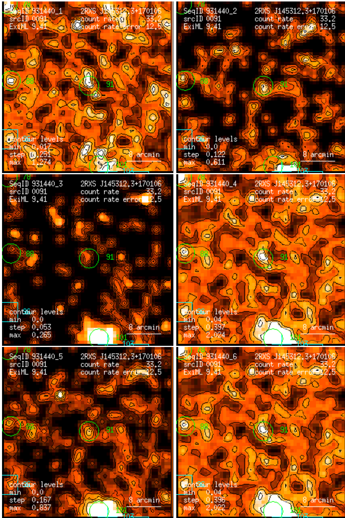
Figure 91: RASS 931440: detection 0091: band rate images, Gaussian filter: (1) PSPC channels 11 – 41, (2) 52 – 90, (3) 91 – 201, (4) 11 – 235, (5) 52 – 201, (6) 11 – 201. Broad band rates in counts/ks. Band rate contour levels in counts/ks/arcmin 2 .
