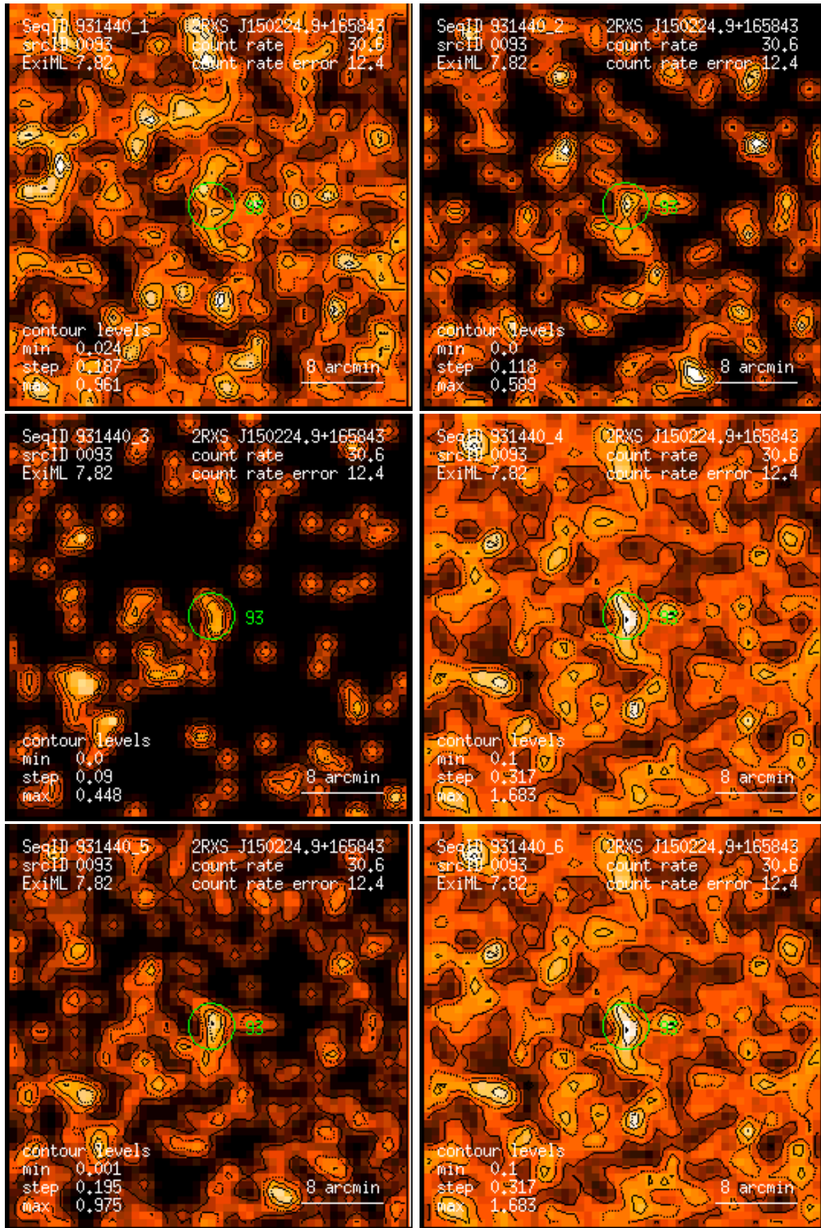
Figure 93: RASS 931440: detection 0093: band rate images, Gaussian filter: (1) PSPC channels 11 – 41, (2) 52 – 90, (3) 91 – 201, (4) 11 – 235, (5) 52 – 201, (6) 11 – 201. Broad band rates in counts/ks. Band rate contour levels in counts/ks/arcmin 2 .
