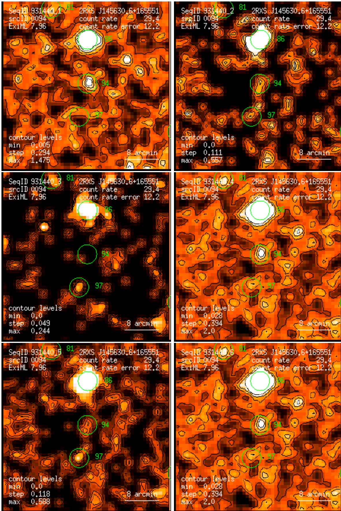
Figure 94: RASS 931440: detection 0094: band rate images, Gaussian filter: (1) PSPC channels 11 – 41, (2) 52 – 90, (3) 91 – 201, (4) 11 – 235, (5) 52 – 201, (6) 11 – 201. Broad band rates in counts/ks. Band rate contour levels in counts/ks/arcmin 2 .
