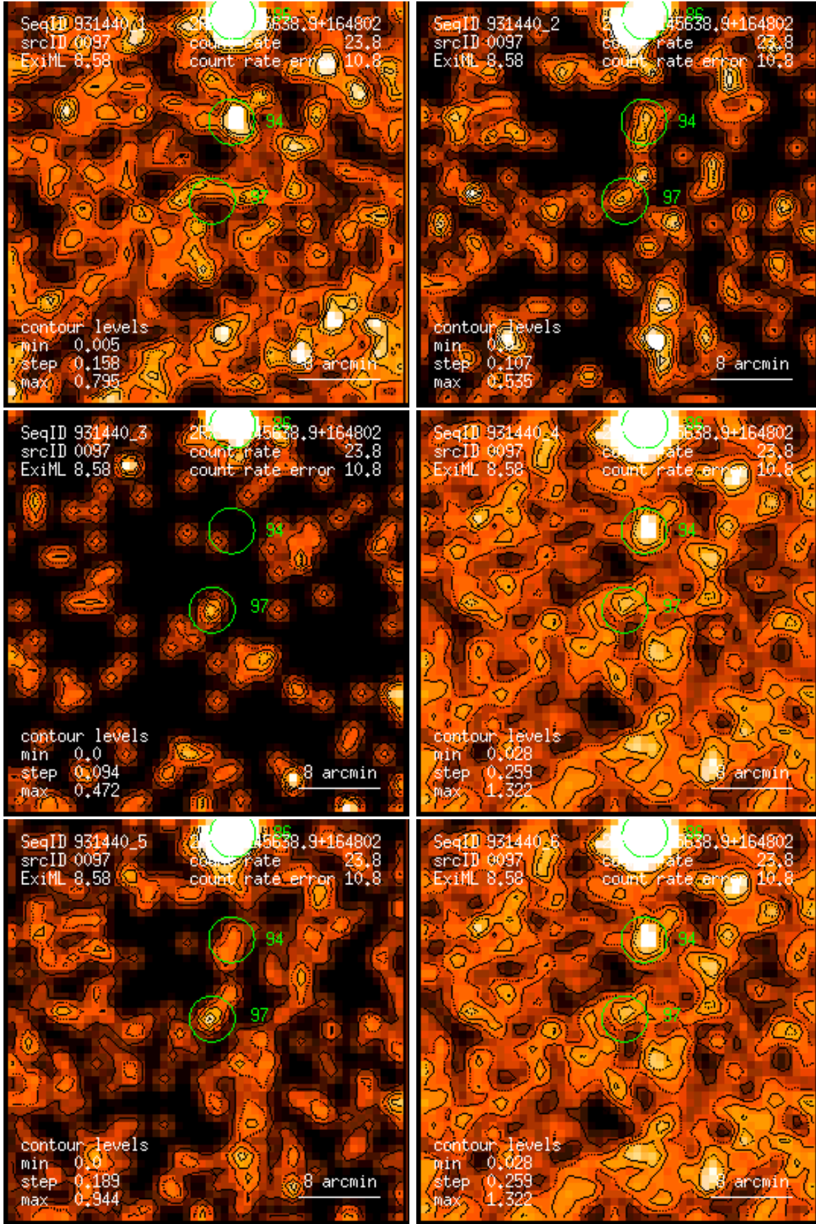
Figure 97: RASS 931440: detection 0097: band rate images, Gaussian filter: (1) PSPC channels 11 – 41, (2) 52 – 90, (3) 91 – 201, (4) 11 – 235, (5) 52 – 201, (6) 11 – 201. Broad band rates in counts/ks. Band rate contour levels in counts/ks/arcmin 2 .
