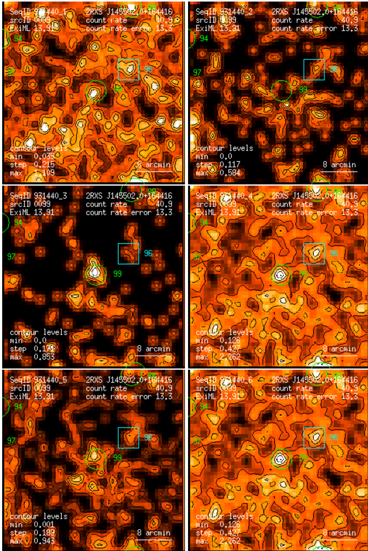
Figure 99: RASS 931440: detection 0099: band rate images, Gaussian filter: (1) PSPC channels 11 – 41, (2) 52 – 90, (3) 91 – 201, (4) 11 – 235, (5) 52 – 201, (6) 11 – 201. Broad band rates in counts/ks. Band rate contour levels in counts/ks/arcmin 2 .
