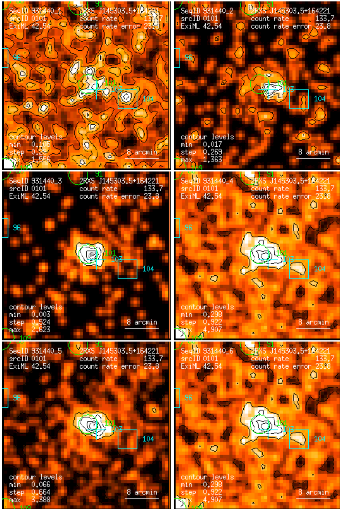
Figure 101: RASS 931440: detection 0101: band rate images, Gaussian filter: (1) PSPC channels 11 – 41, (2) 52 – 90, (3) 91 – 201, (4) 11 – 235, (5) 52 – 201, (6) 11 – 201. Broad band rates in counts/ks. Band rate contour levels in counts/ks/arcmin 2 .
