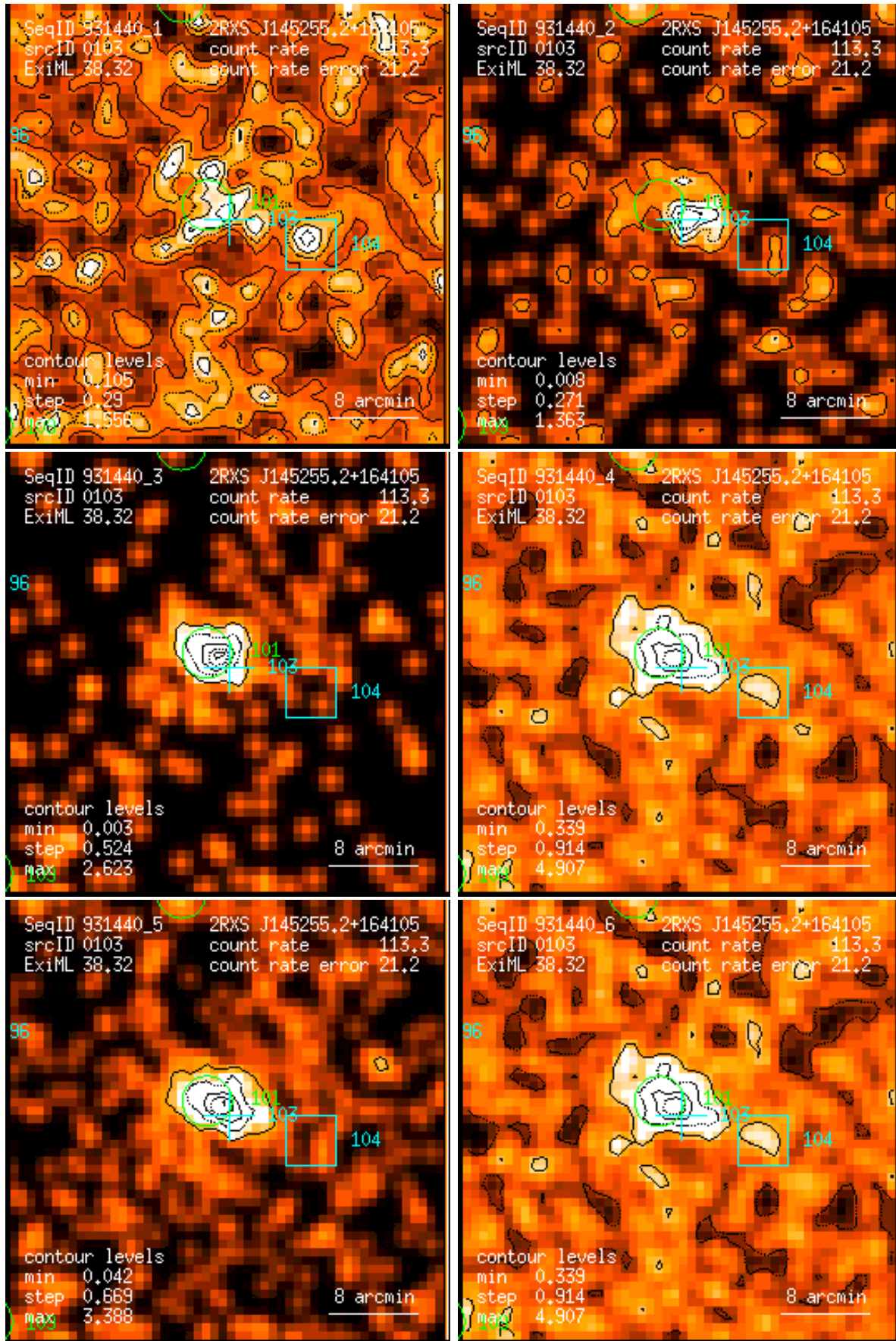
Figure 103: RASS 931440: detection 0103: band rate images, Gaussian filter: (1) PSPC channels 11 – 41, (2) 52 – 90, (3) 91 – 201, (4) 11 – 235, (5) 52 – 201, (6) 11 – 201. Broad band rates in counts/ks. Band rate contour levels in counts/ks/arcmin 2 .
