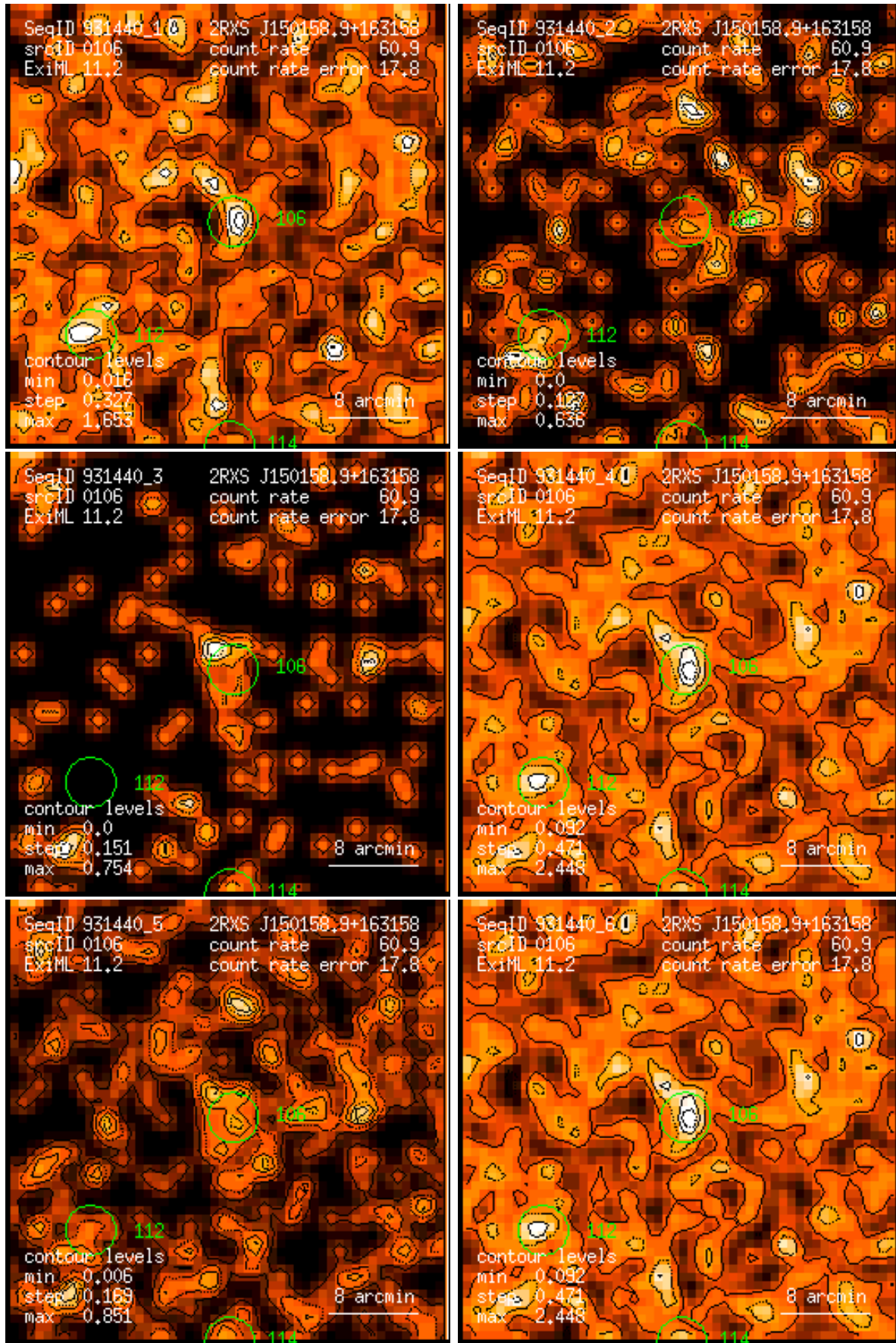
Figure 106: RASS 931440: detection 0106: band rate images, Gaussian filter: (1) PSPC channels 11 – 41, (2) 52 – 90, (3) 91 – 201, (4) 11 – 235, (5) 52 – 201, (6) 11 – 201. Broad band rates in counts/ks. Band rate contour levels in counts/ks/arcmin 2 .
