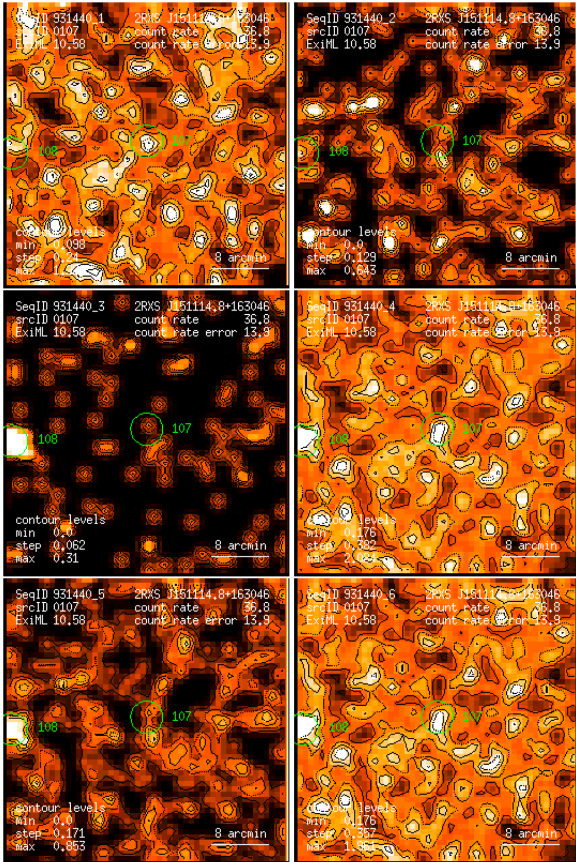
Figure 107: RASS 931440: detection 0107: band rate images, Gaussian filter: (1) PSPPC channels 11 – 41, (2) 52 – 90, (3) 91 – 201, (4) 11 – 235, (5) 52 – 201, (6) 11 – 201. Broad band rates in counts/ks. Band rate contour levels in counts/ks/arcmin 2 .
