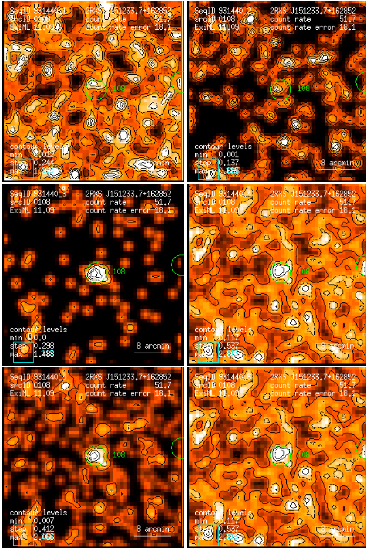
Figure 108: RASS 931440: detection 0108: band rate images, Gaussian filter: (1) PSPC channels 11 – 41, (2) 52 – 90, (3) 91 – 201, (4) 11 – 235, (5) 52 – 201, (6) 11 – 201. Broad band rates in counts/ks. Band rate contour levels in counts/ks/arcmin 2 .
