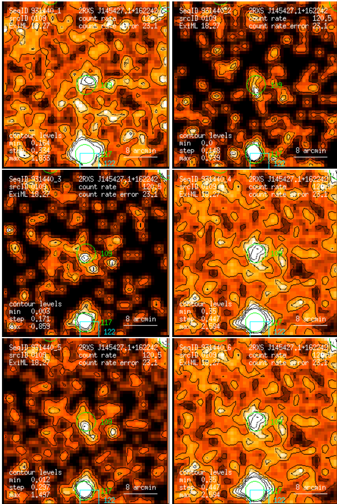
Figure 109: RASS 931440: detection 0109: band rate images, Gaussian filter: (1) PSPC channels 11 – 41, (2) 52 – 90, (3) 91 – 201, (4) 11 – 235, (5) 52 – 201, (6) 11 – 201. Broad band rates in counts/ks. Band rate contour levels in counts/ks/arcmin 2 .
