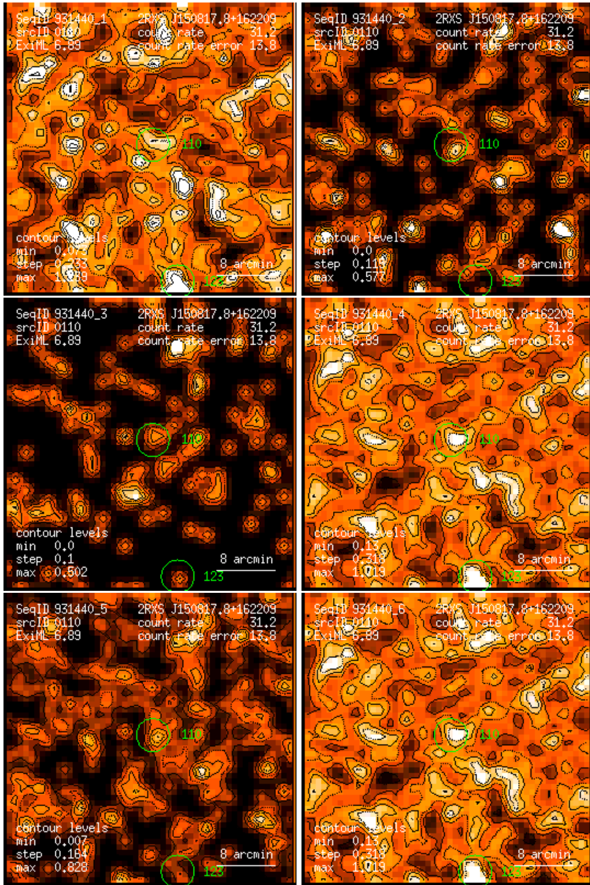
Figure 110: RASS 931440: detection 0110: band rate images, Gaussian filter: (1) PSPC channels 11 – 41, (2) 52 – 90, (3) 91 – 201, (4) 11 – 235, (5) 52 – 201, (6) 11 – 201. Broad band rates in counts/ks. Band rate contour levels in counts/ks/arcmin 2 .
