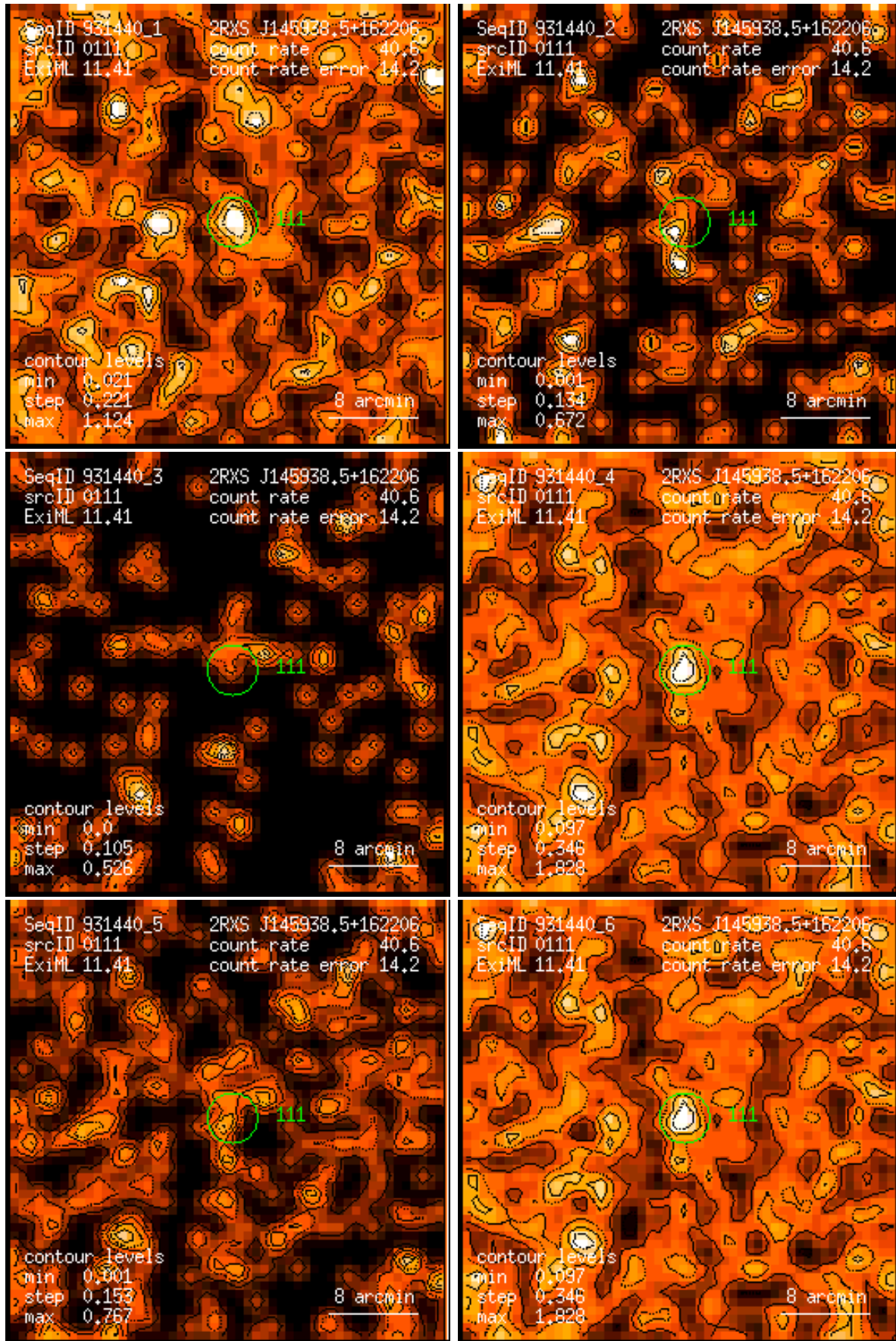
Figure 111: RASS 931440: detection 0111: band rate images, Gaussian filter: (1) PSPC channels 11 – 41, (2) 52 – 90, (3) 91 – 201, (4) 11 – 235, (5) 52 – 201, (6) 11 – 201. Broad band rates in counts/ks. Band rate contour levels in counts/ks/arcmin 2 .
