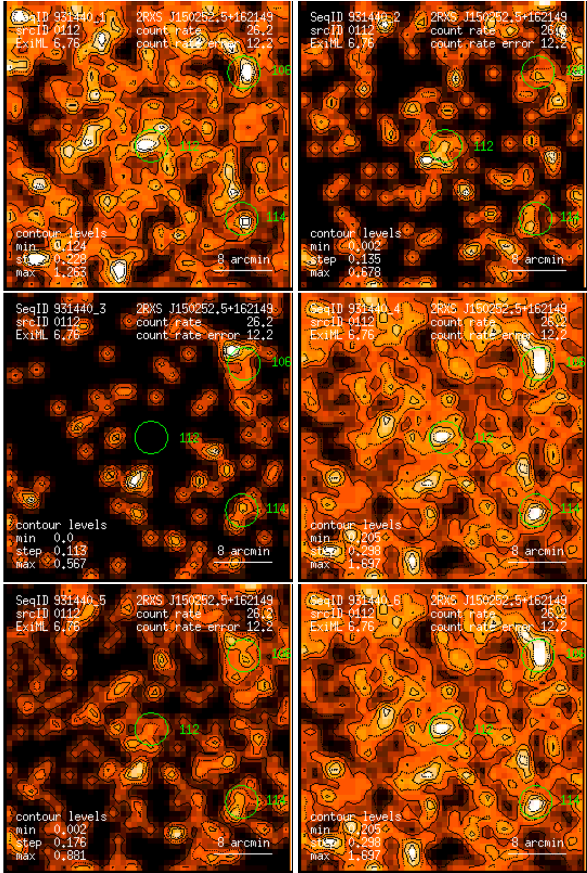
Figure 112: RASS 931440: detection 0112: band rate images, Gaussian filter: (1) PSPC channels 11 – 41, (2) 52 – 90, (3) 91 – 201, (4) 11 – 235, (5) 52 – 201, (6) 11 – 201. Broad band rates in counts/ks. Band rate contour levels in counts/ks/arcmin 2 .
