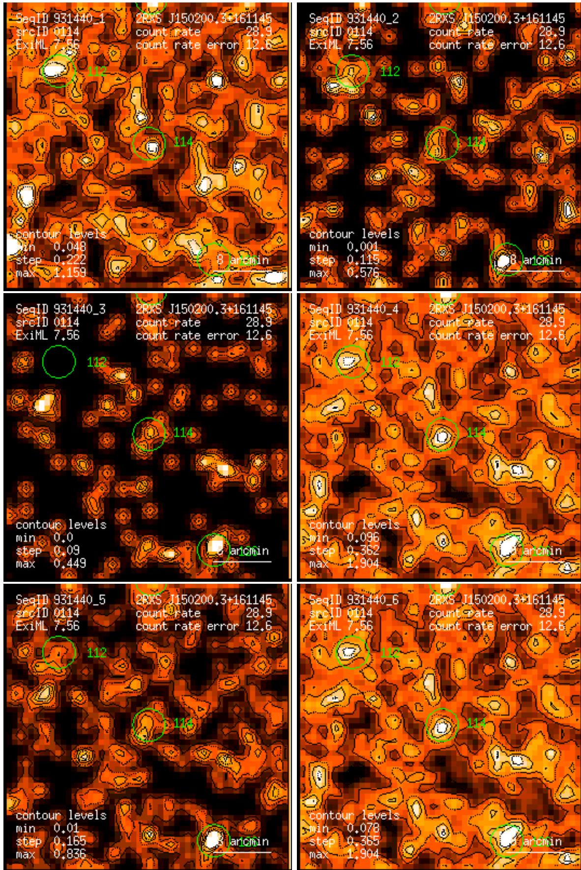
Figure 114: RASS 931440: detection 0114: band rate images, Gaussian filter: (1) PSPC channels 11 – 41, (2) 52 – 90, (3) 91 – 201, (4) 11 – 235, (5) 52 – 201, (6) 11 – 201. Broad band rates in counts/ks. Band rate contour levels in counts/ks/arcmin 2 .
