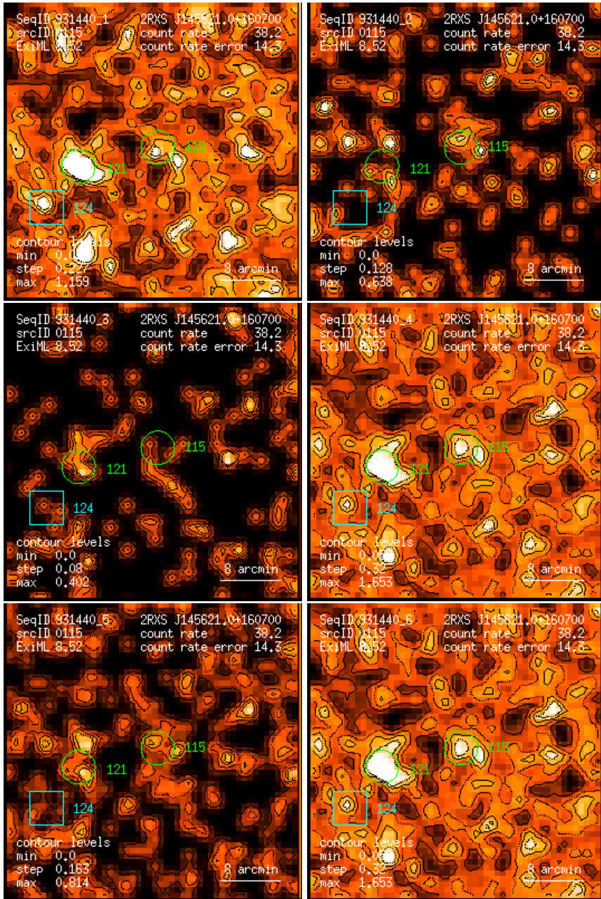
Figure 115: RASS 931440: detection 0115: band rate images, Gaussian filter: (1) PSPC channels 11 – 41, (2) 52 – 90, (3) 91 – 201, (4) 11 – 235, (5) 52 – 201, (6) 11 – 201. Broad band rates in counts/ks. Band rate contour levels in counts/ks/arcmin 2 .
