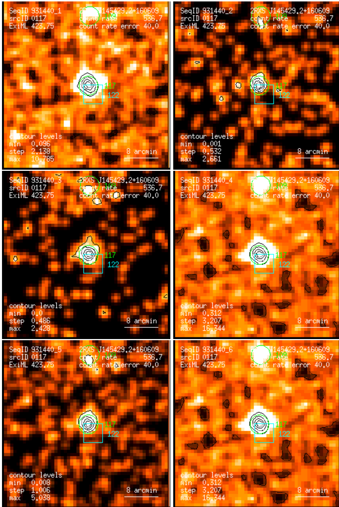
Figure 117: RASS 931440: detection 0117: band rate images, Gaussian filter: (1) PSPC channels 11 – 41, (2) 52 – 90, (3) 91 – 201, (4) 11 – 235, (5) 52 – 201, (6) 11 – 201. Broad band rates in counts/ks. Band rate contour levels in counts/ks/arcmin 2 .
