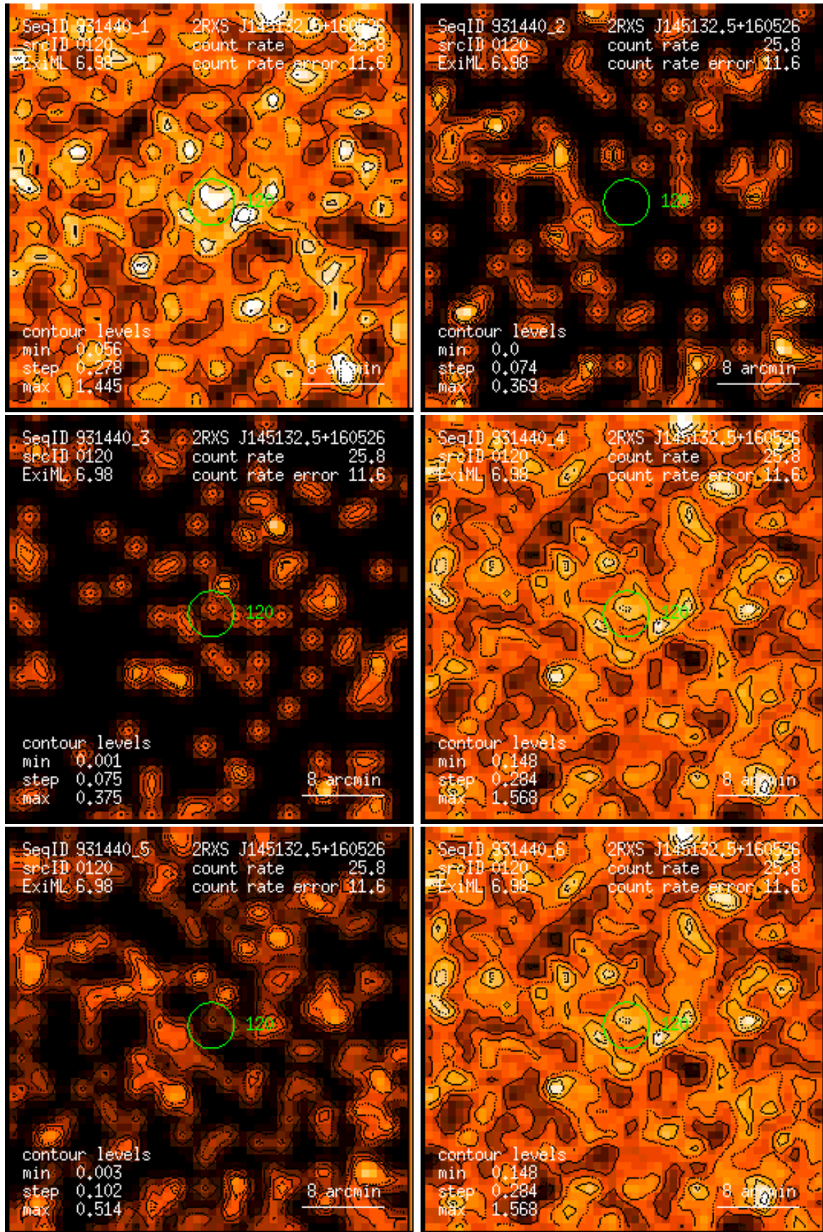
Figure 120: RASS 931440: detection 0120: band rate images, Gaussian filter: (1) PSPC channels 11 – 41, (2) 52 – 90, (3) 91 – 201, (4) 11 – 235, (5) 52 – 201, (6) 11 – 201. Broad band rates in counts/ks. Band rate contour levels in counts/ks/arcmin 2 .
