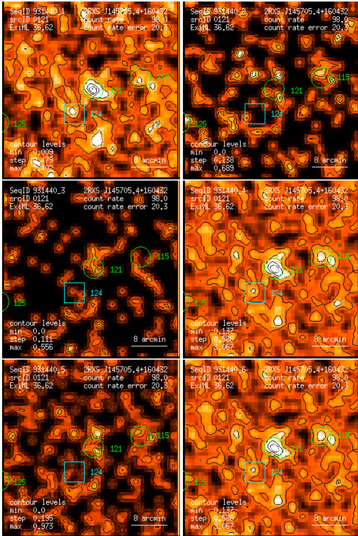
Figure 121: RASS 931440: detection 0121: band rate images, Gaussian filter: (1) PSPC channels 11 – 41, (2) 52 – 90, (3) 91 – 201, (4) 11 – 235, (5) 52 – 201, (6) 11 – 201. Broad band rates in counts/ks. Band rate contour levels in counts/ks/arcmin 2 .
