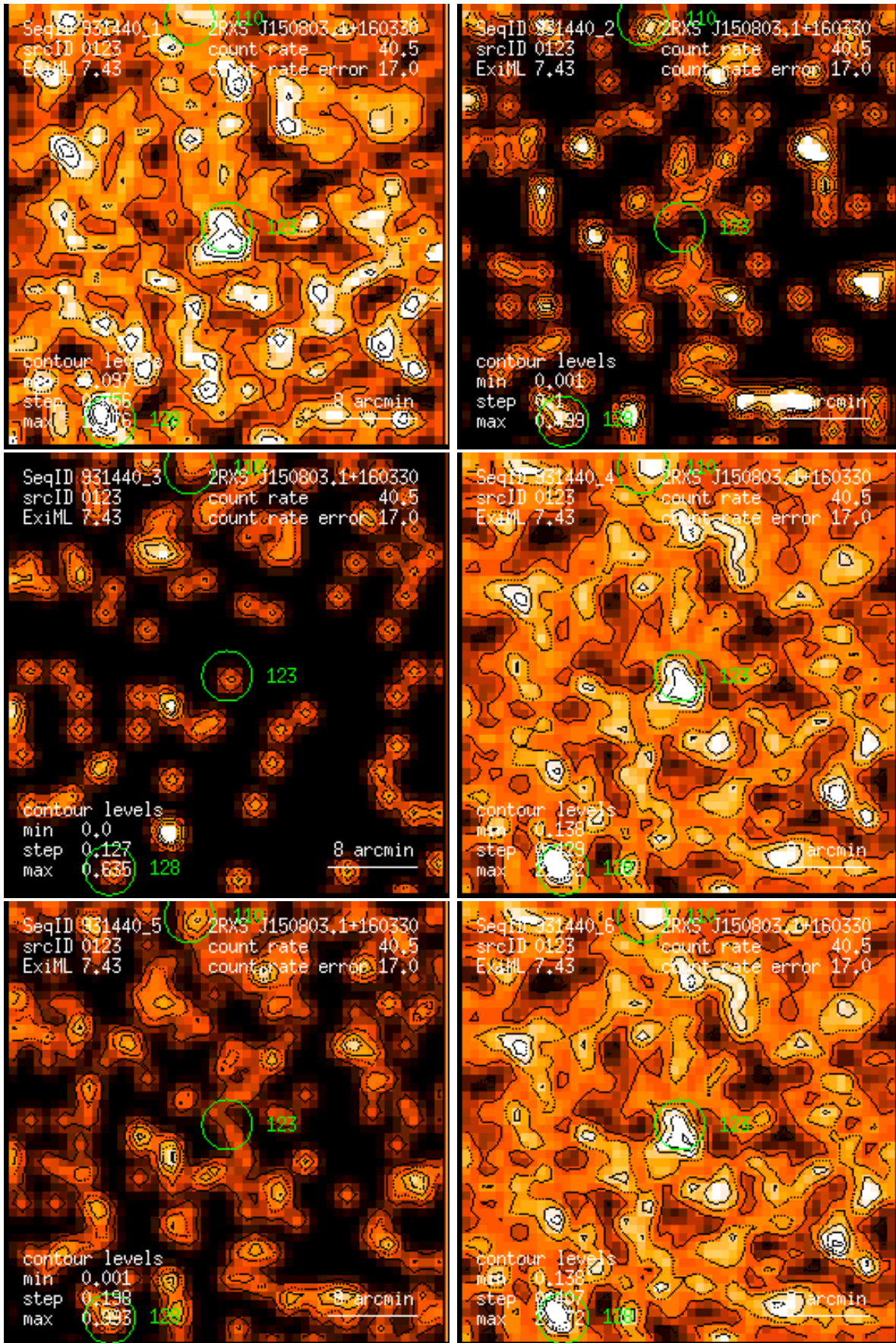
Figure 123: RASS 931440: detection 0123: band rate images, Gaussian filter: (1) PSPC channels 11 – 41, (2) 52 – 90, (3) 91 – 201, (4) 11 – 235, (5) 52 – 201, (6) 11 – 201. Broad band rates in counts/ks. Band rate contour levels in counts/ks/arcmin 2 .
