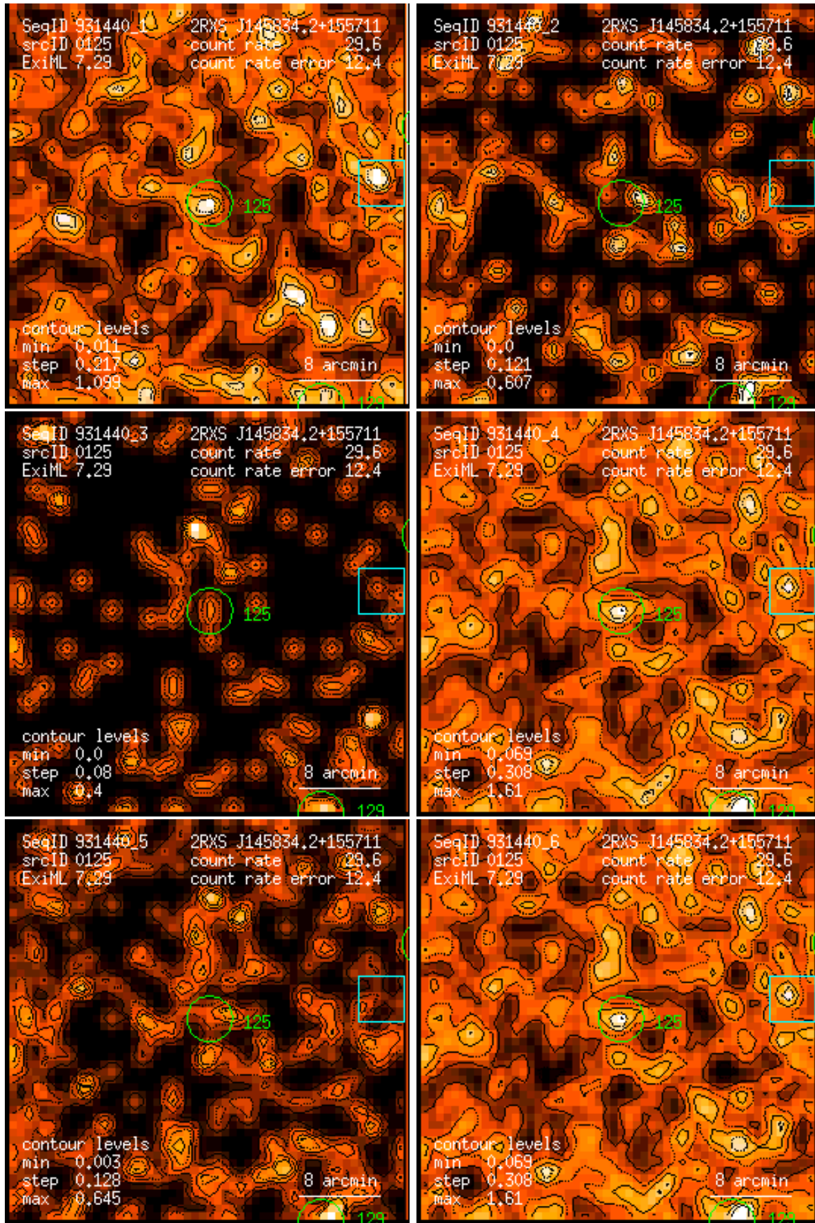
Figure 125: RASS 931440: detection 0125: band rate images, Gaussian filter: (1) PSPC channels 11 – 41, (2) 52 – 90, (3) 91 – 201, (4) 11 – 235, (5) 52 – 201, (6) 11 – 201. Broad band rates in counts/ks. Band rate contour levels in counts/ks/arcmin 2 .
