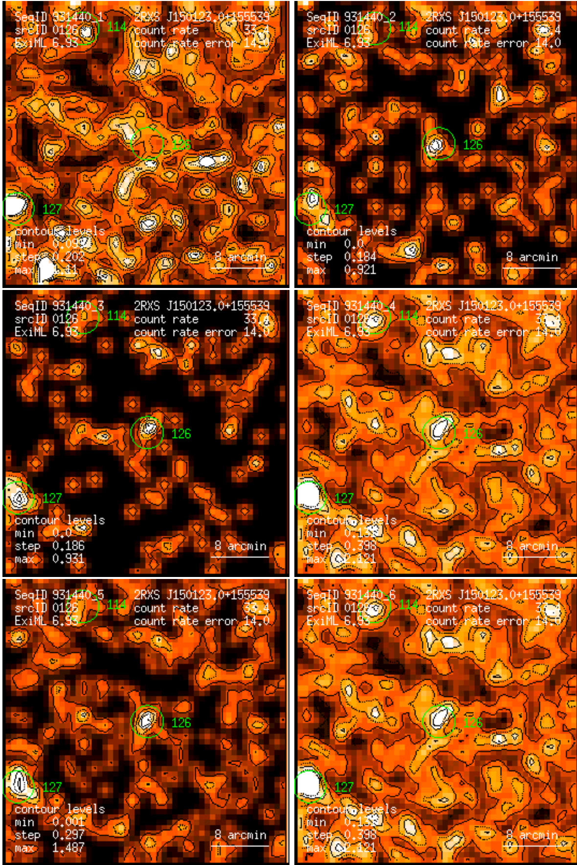
Figure 126: RASS 931440: detection 0126: band rate images, Gaussian filter: (1) PSPC channels 11 – 41, (2) 52 – 90, (3) 91 – 201, (4) 11 – 235, (5) 52 – 201, (6) 11 – 201. Broad band rates in counts/ks. Band rate contour levels in counts/ks/arcmin 2 .
